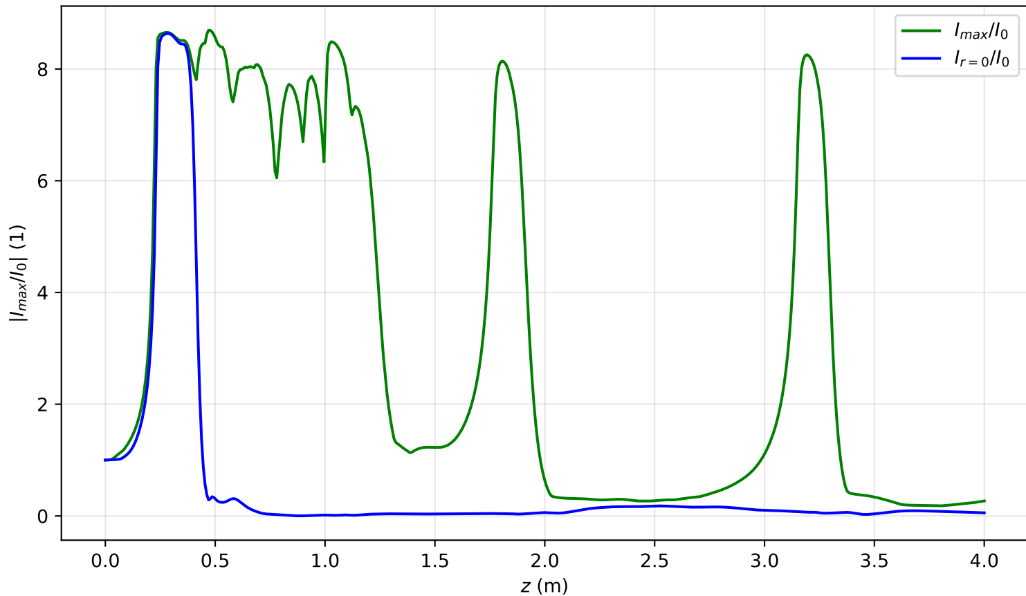
I_{max}(x = 0, y = 0, z)/I_0 , P_{in}=12.9\text{Pcr} , noisy input, artificial time
