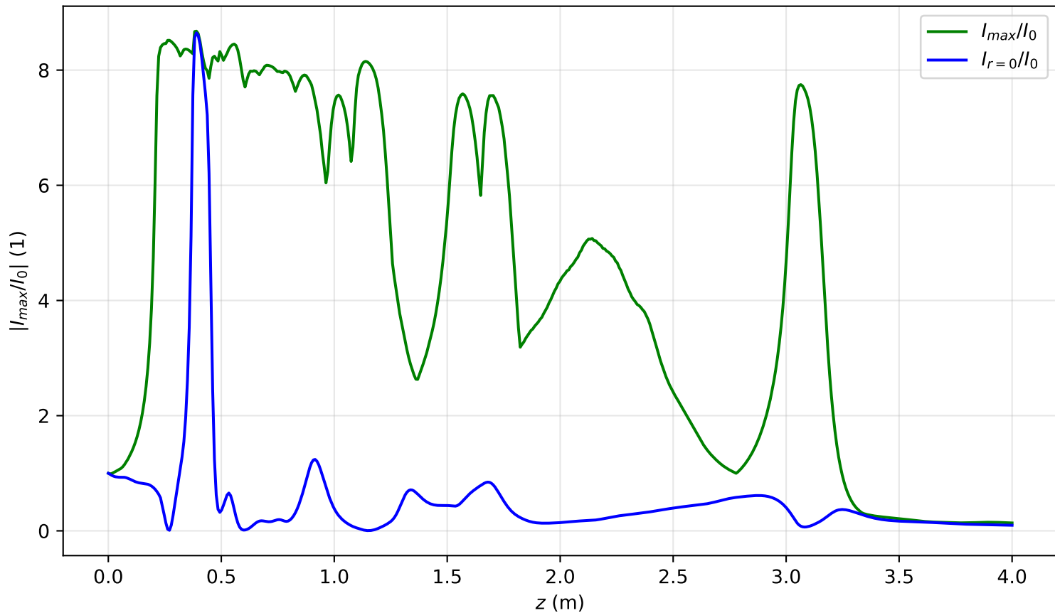
I_{max}(x = 0, y = 0, z)/I_0 , Pin=13.0Pcr, noisy input, artificial time
