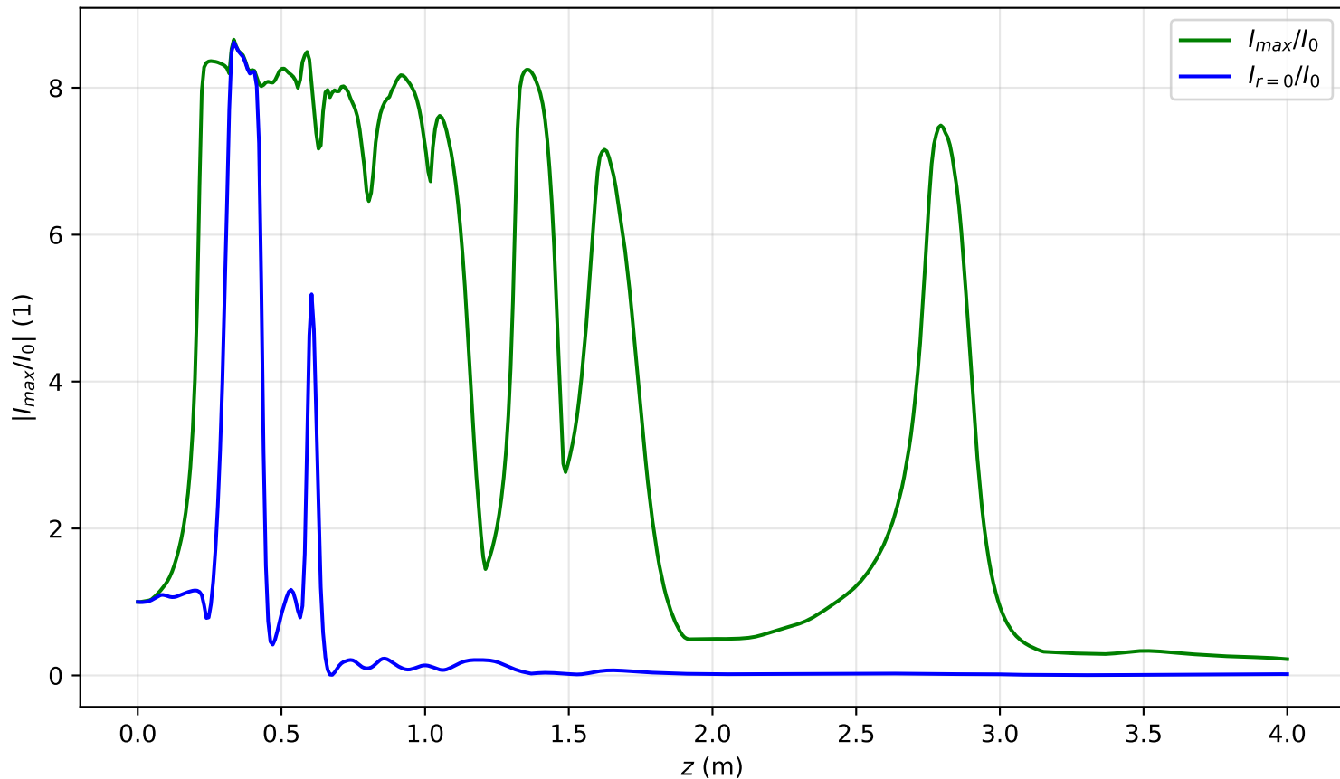
I_{\max}(x = 0, y = 0, z)/I_0 , Pin=13.1Pcr, noisy input, artificial time
