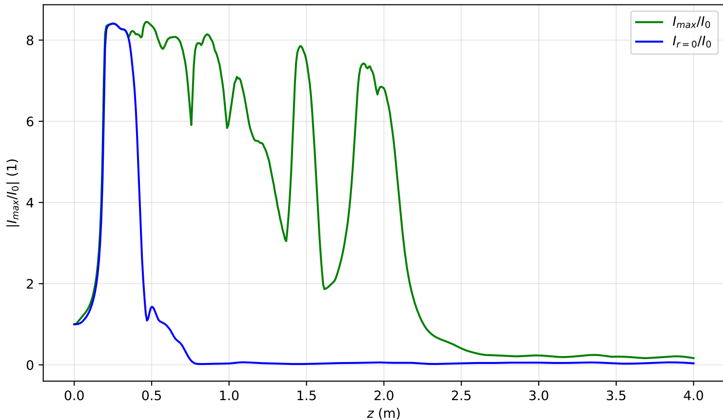
I_{max}(x = 0, y = 0, z)/I_0 , Pin=13.2Pcr, noisy input, artificial time
