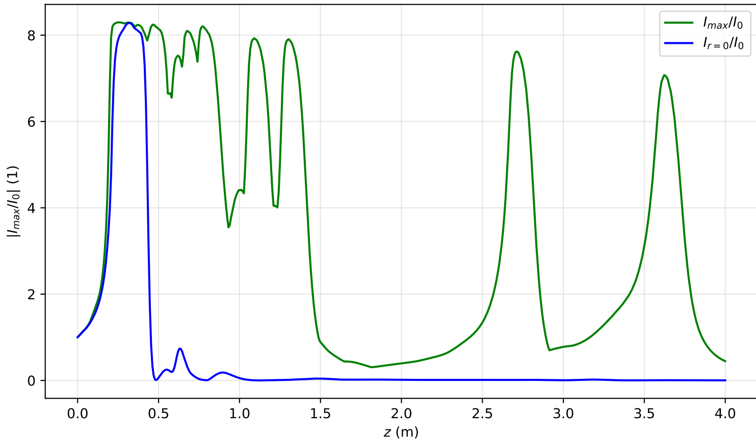
I_{max}(x = 0, y = 0, z)/I_0 , Pin=13.3Pcr, noisy input, artificial time
