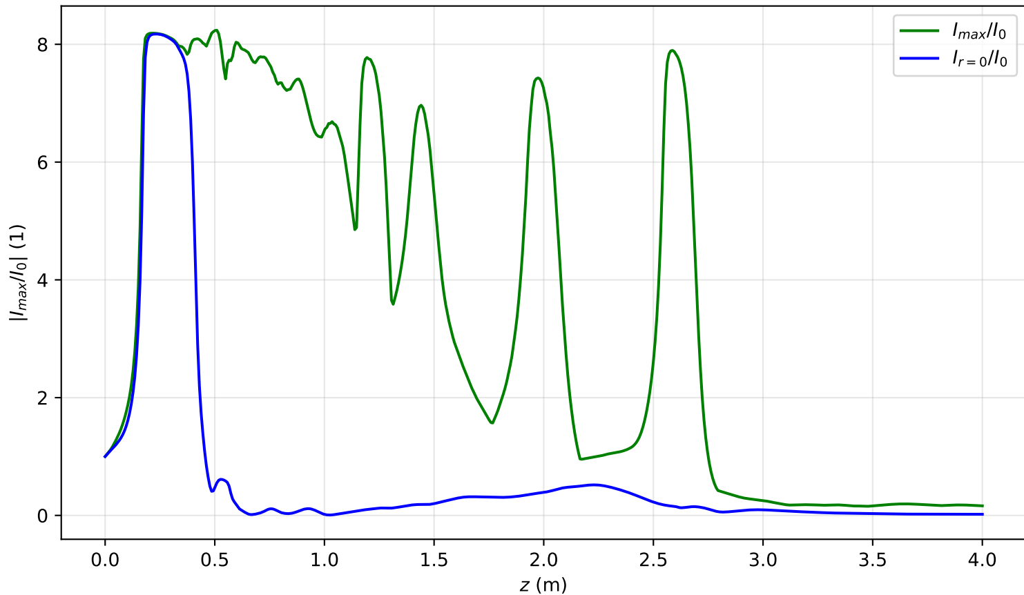
I_{max}(x = 0, y = 0, z)/I_0 , Pin=13.5Pcr, noisy input, artificial time
