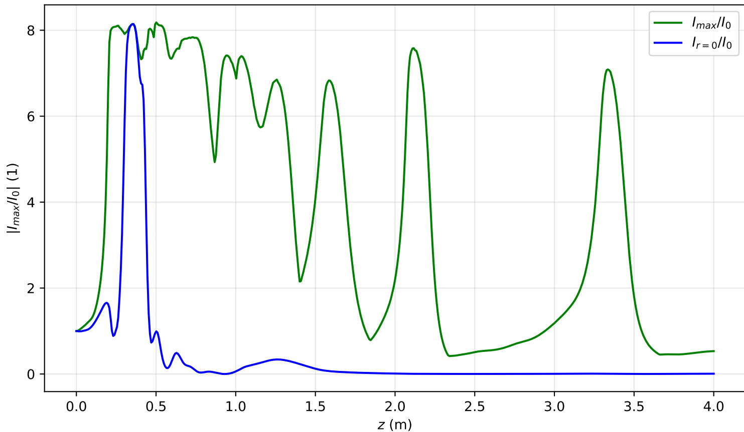
I_{max}(x = 0, y = 0, z)/I_0 , Pin=13.6Pcr, noisy input, artificial time
