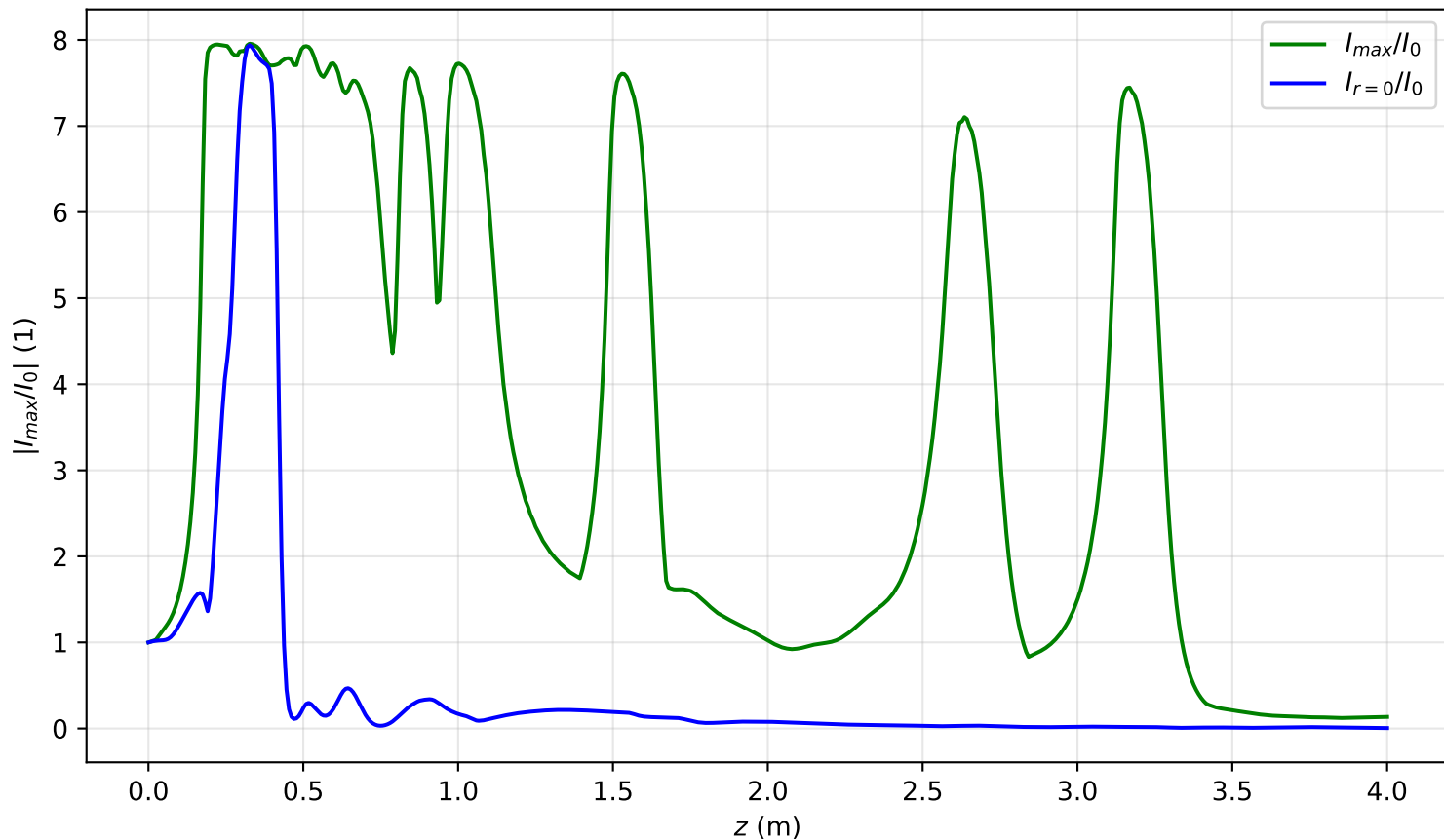
I_{max}(x = 0, y = 0, z)/I_0 , Pin=13.8Pcr, noisy input, artificial time
