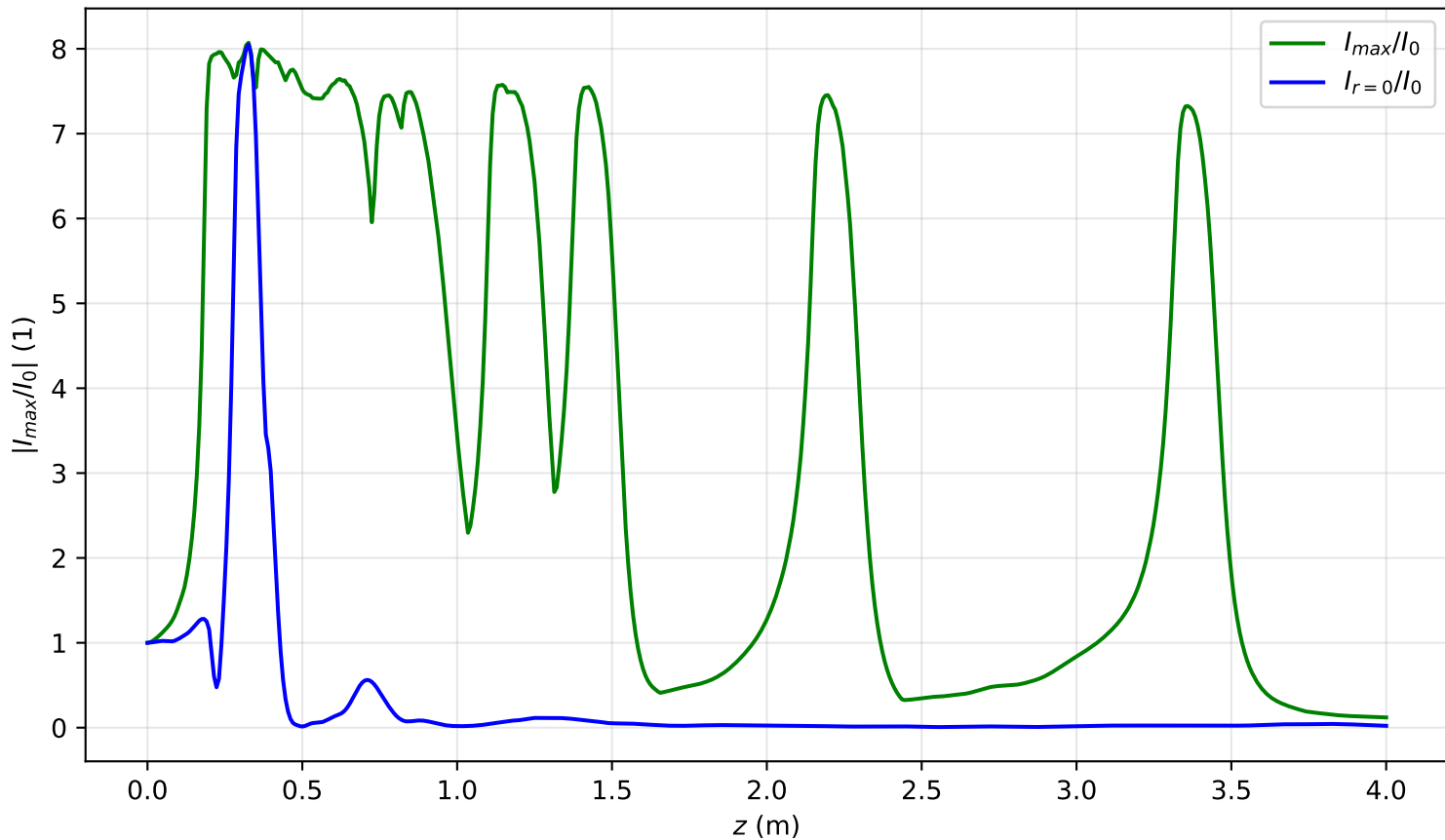
I_{max}(x = 0, y = 0, z)/I_0 , P_{in}=13.9\text{Pcr} , noisy input, artificial time
