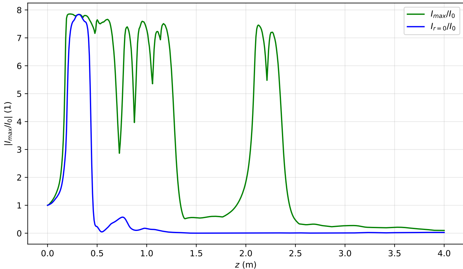
I_{max}(x = 0, y = 0, z)/I_0 , Pin=14.0Pcr, noisy input, artificial time
