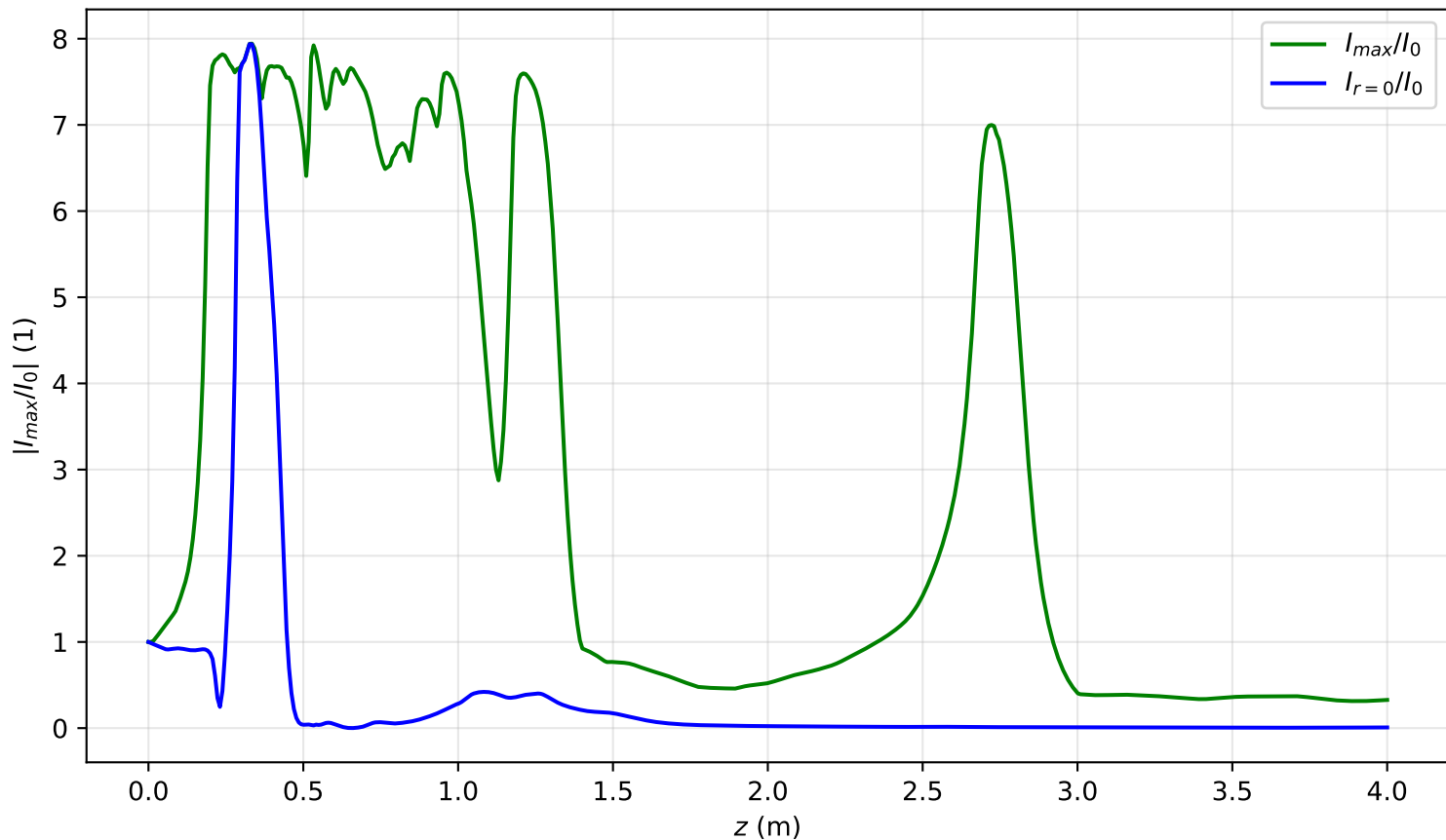
I_{max}(x = 0, y = 0, z)/I_0 , P_{in}=14.1\text{Pcr} , noisy input, artificial time
