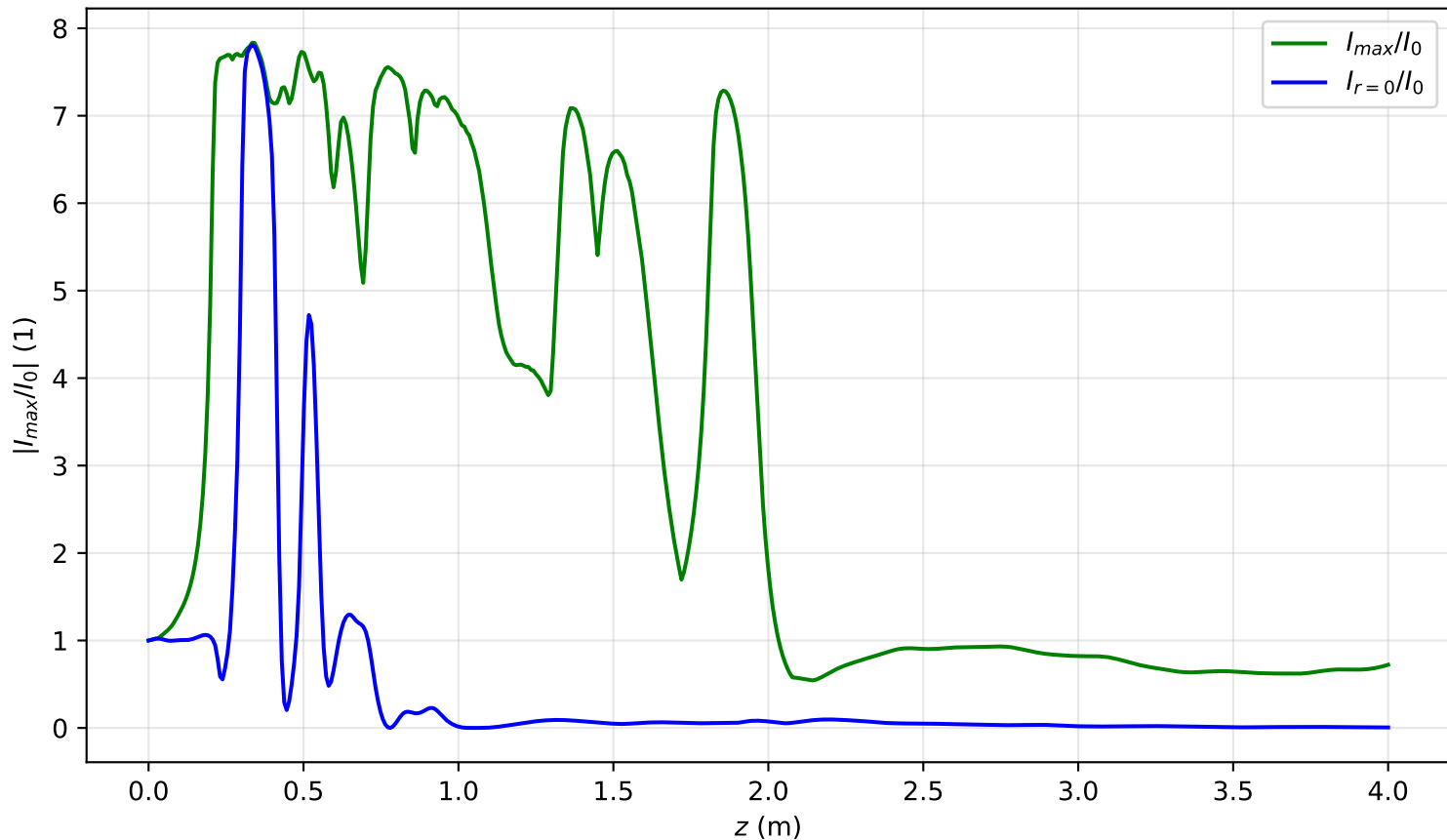
I_{max}(x = 0, y = 0, z)/I_0 , Pin=14.3Pcr, noisy input, artificial time
