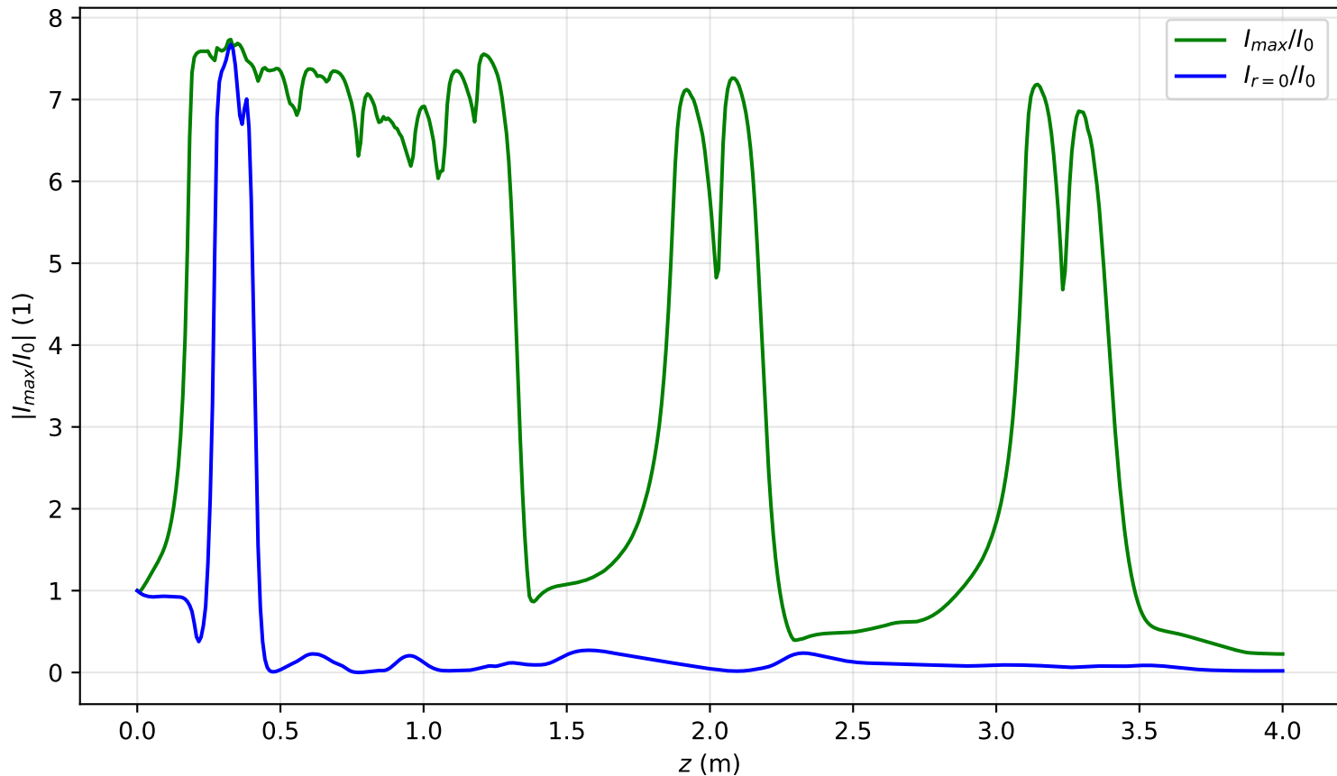
I_{max}(x = 0, y = 0, z)/I_0 , Pin=14.4Pcr, noisy input, artificial time
