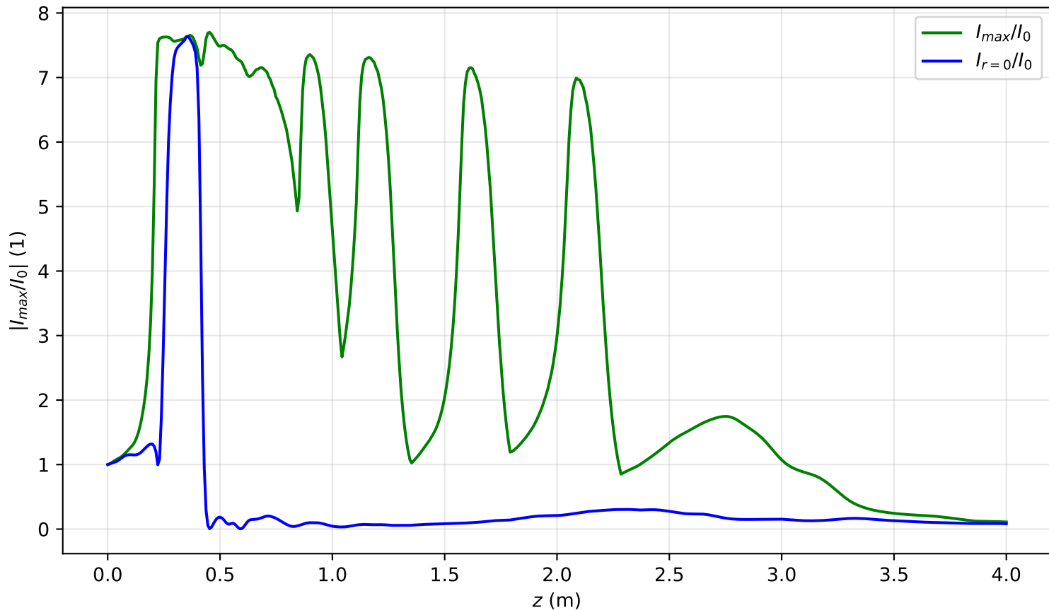
I_{max}(x = 0, y = 0, z)/I_0 , Pin=14.5Pcr, noisy input, artificial time
