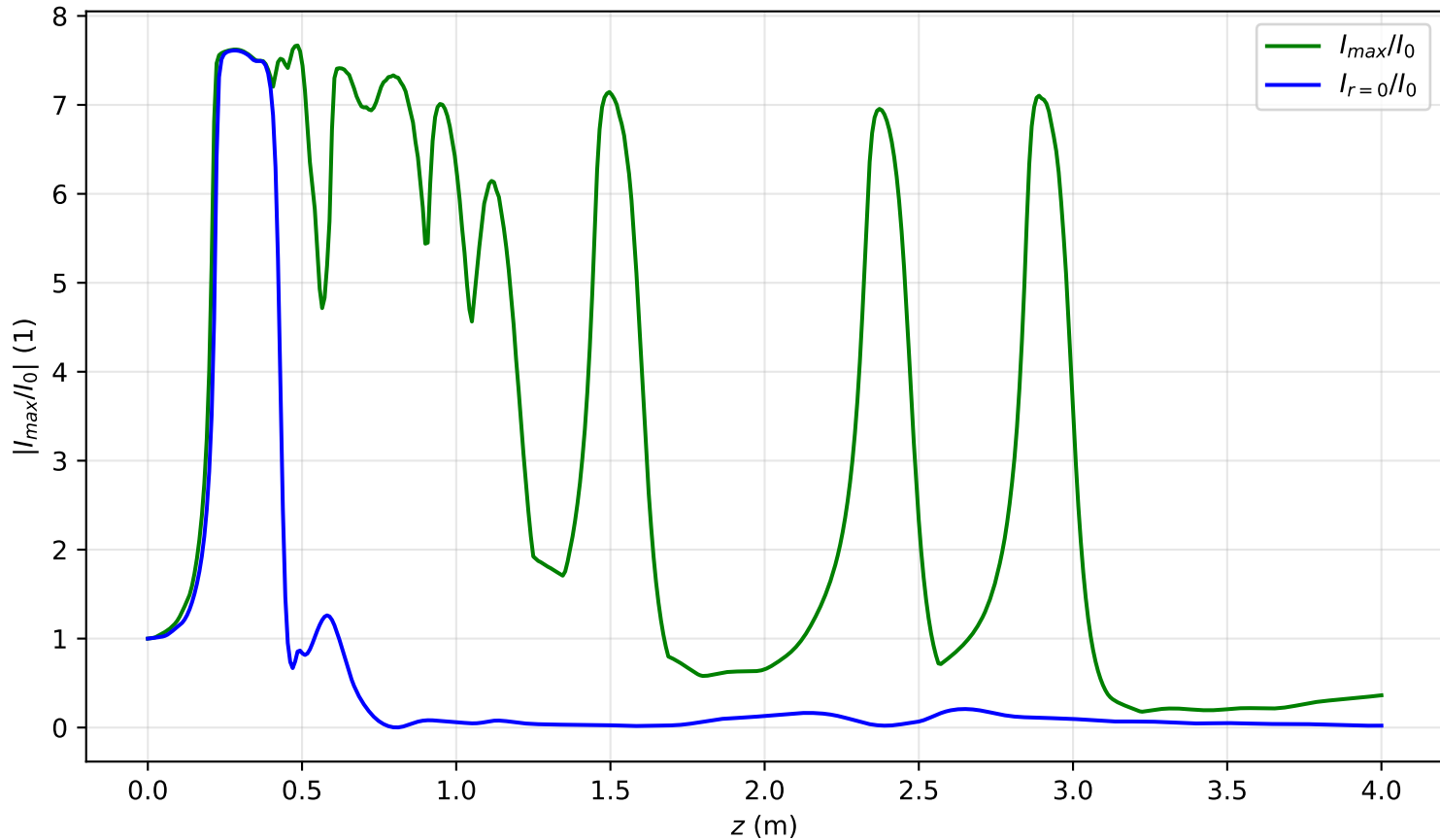
I_{max}(x = 0, y = 0, z)/I_0 , Pin=14.6Pcr, noisy input, artificial time
