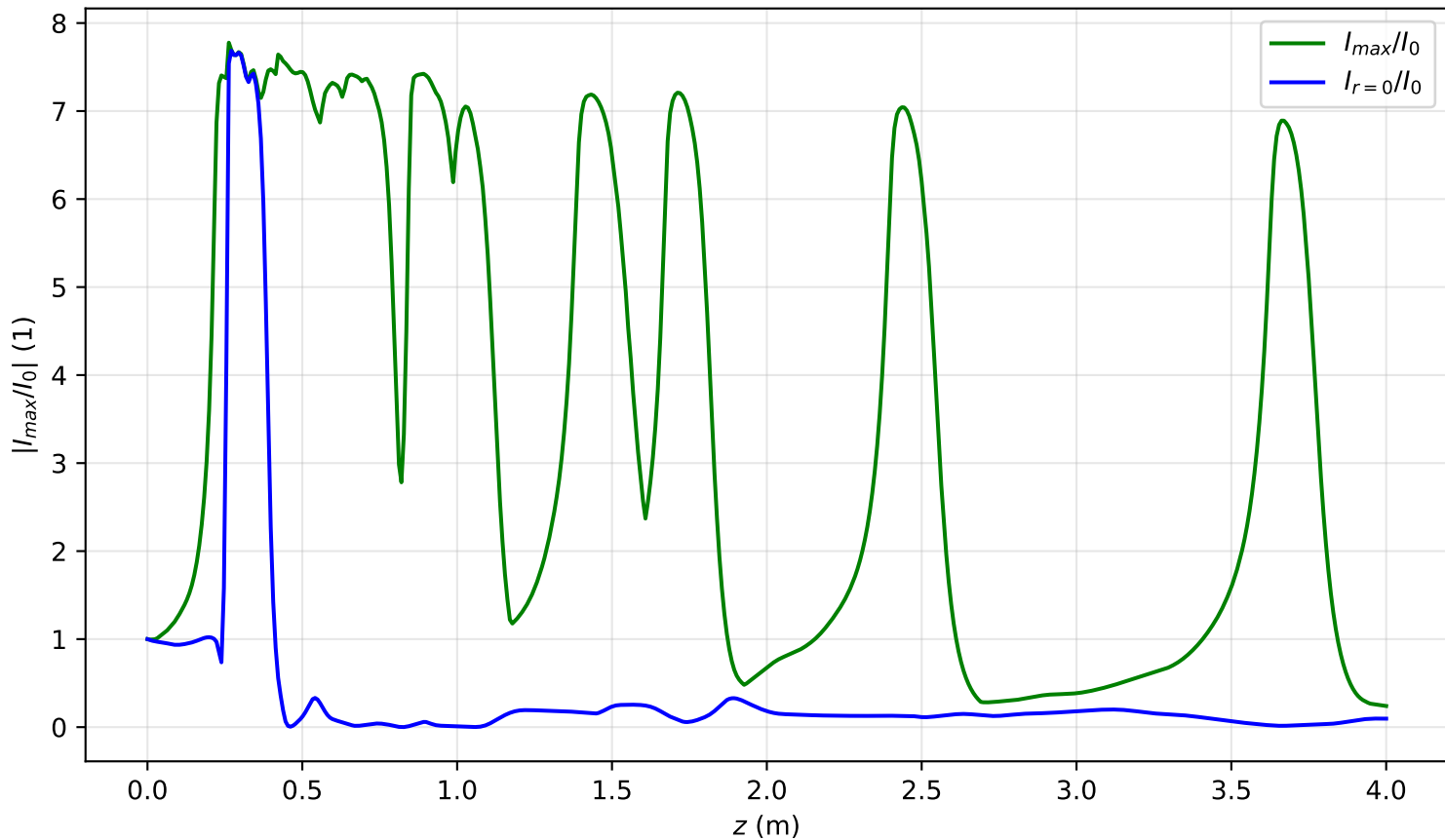
I_{max}(x = 0, y = 0, z)/I_0 , P_{in}=14.7\text{Pcr} , noisy input, artificial time
