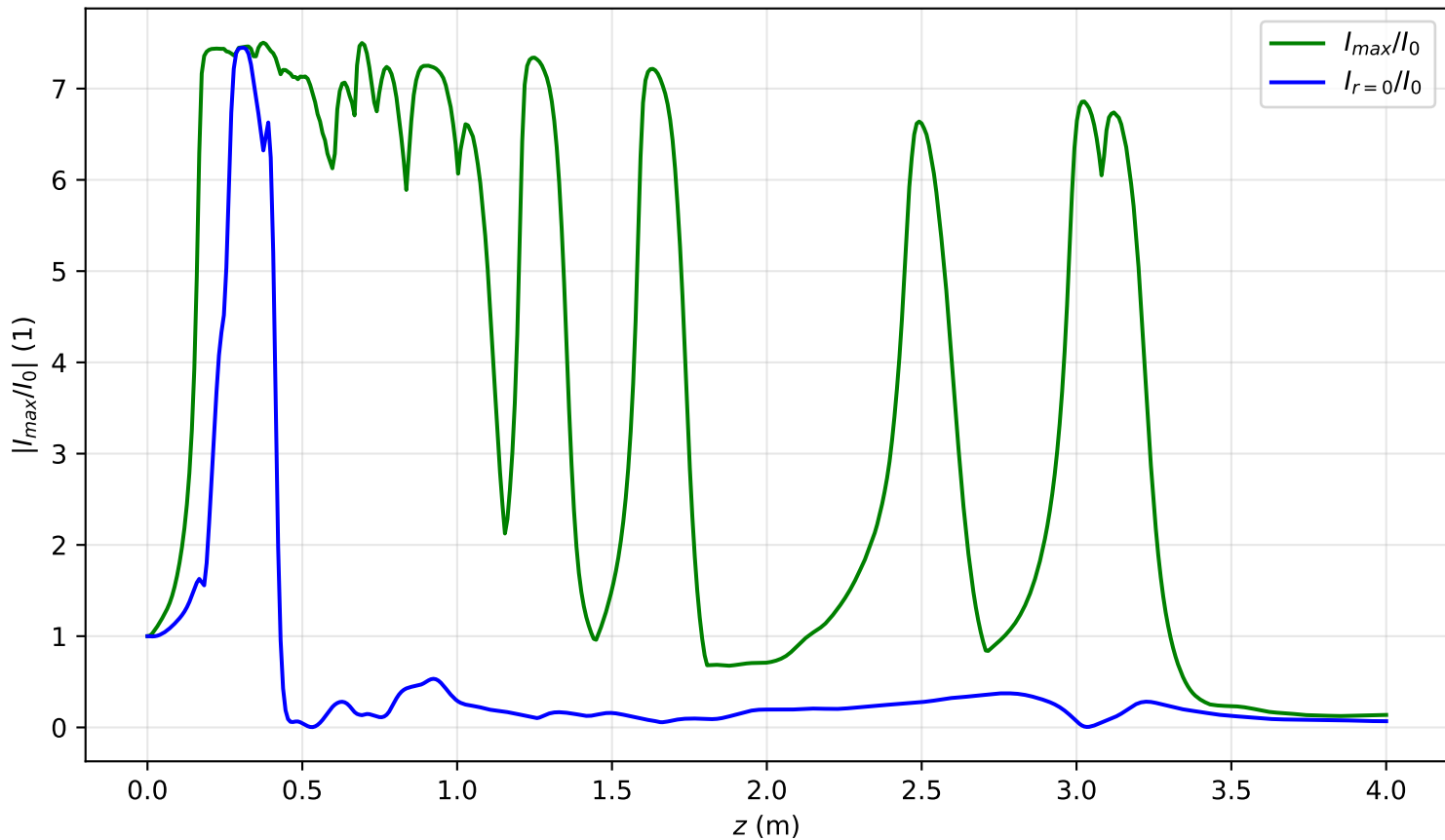
I_{\max}(x = 0, y = 0, z)/I_0 , P_{\text{in}}=14.8\text{Pcr} , noisy input, artificial time
