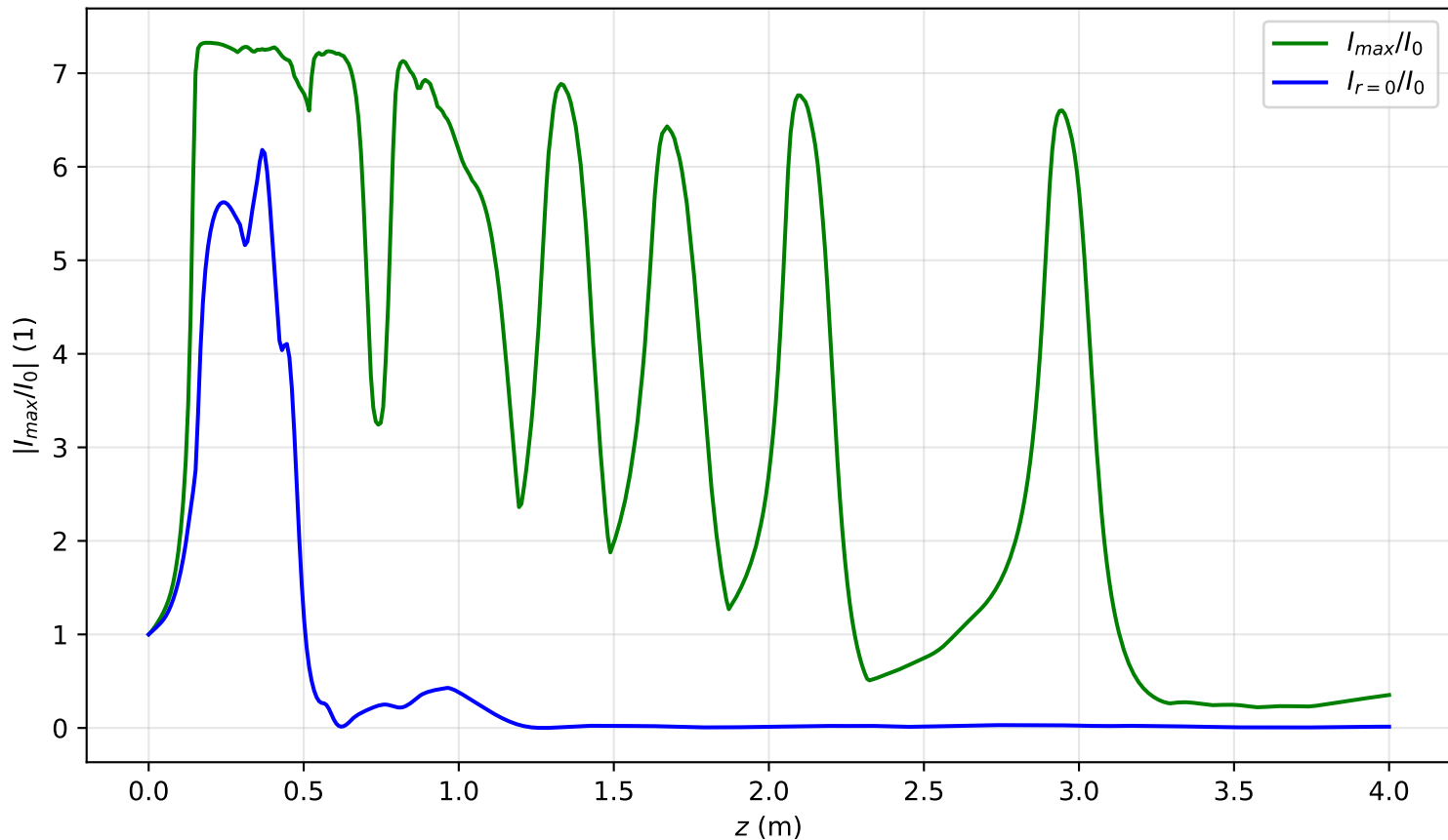
I_{max}(x = 0, y = 0, z)/I_0 , Pin=15.1Pcr, noisy input, artificial time
