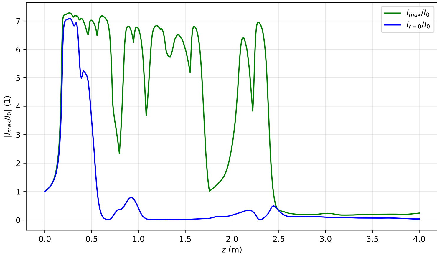
I_{max}(x = 0, y = 0, z)/I_0 , Pin=15.2Pcr, noisy input, artificial time
