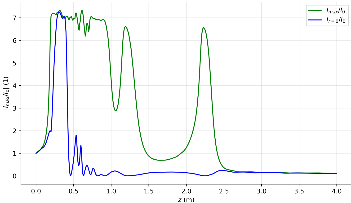
I_{max}(x = 0, y = 0, z)/I_0 , P_{in}=15.3\text{Pcr} , noisy input, artificial time
