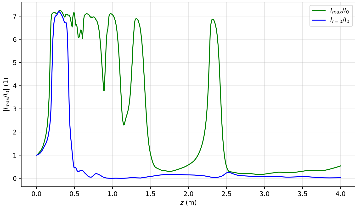
I_{max}(x = 0, y = 0, z)/I_0 , P_{in}=15.4P_{cr} , noisy input, artificial time
