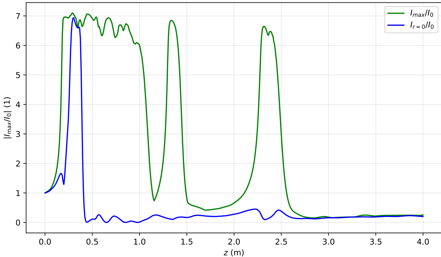
I_{max}(x = 0, y = 0, z)/I_0 , P_{in}=15.7\text{Pcr} , noisy input, artificial time
