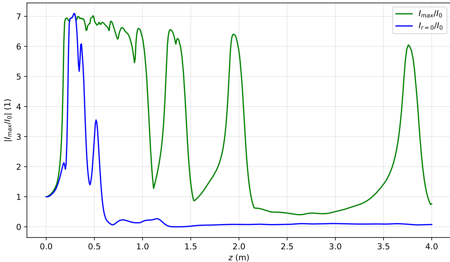
I_{\max}(x = 0, y = 0, z)/I_0 , Pin=15.8Pcr, noisy input, artificial time
