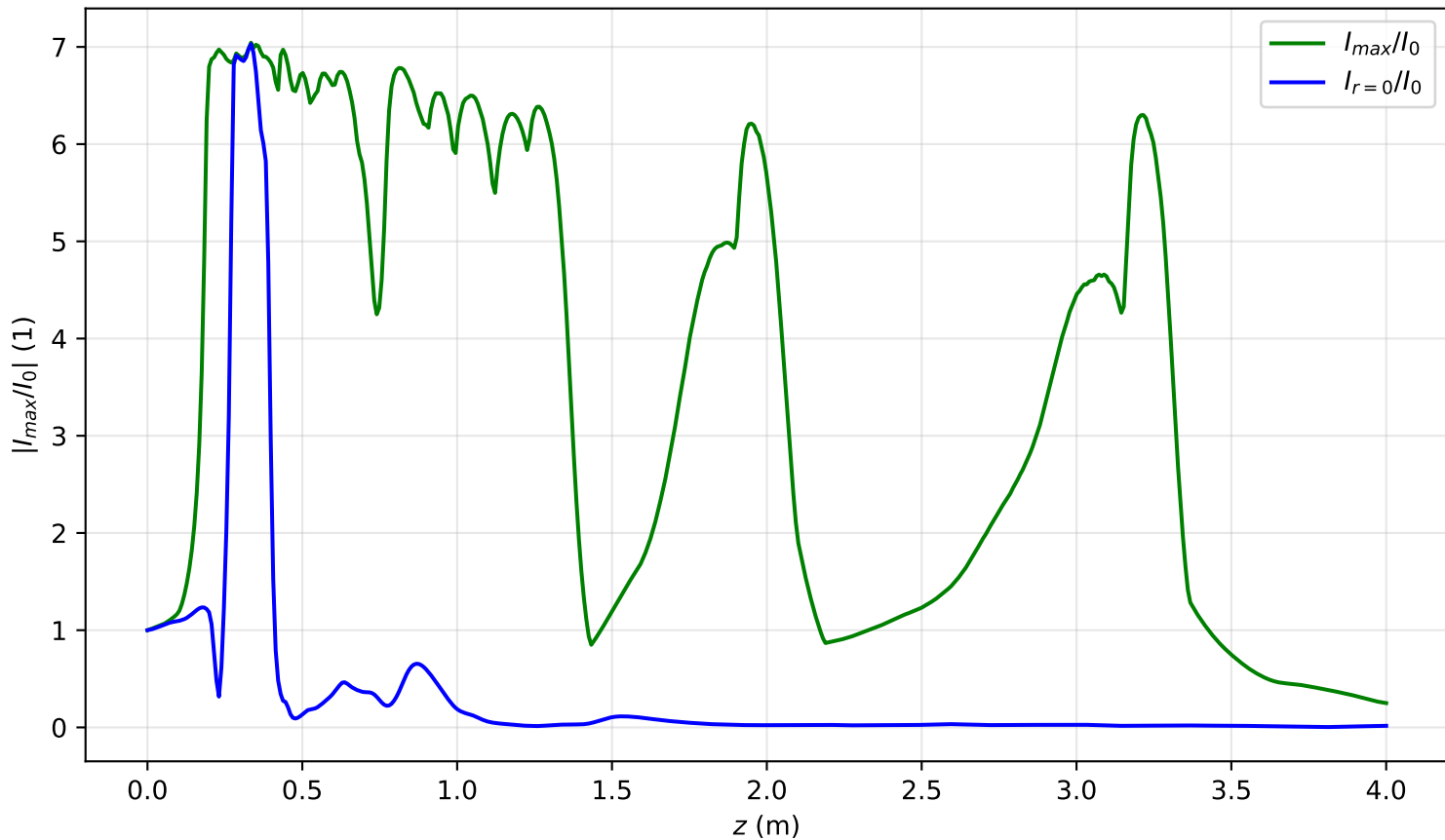
I_{max}(x = 0, y = 0, z)/I_0 , Pin=16.0Pcr, noisy input, artificial time
