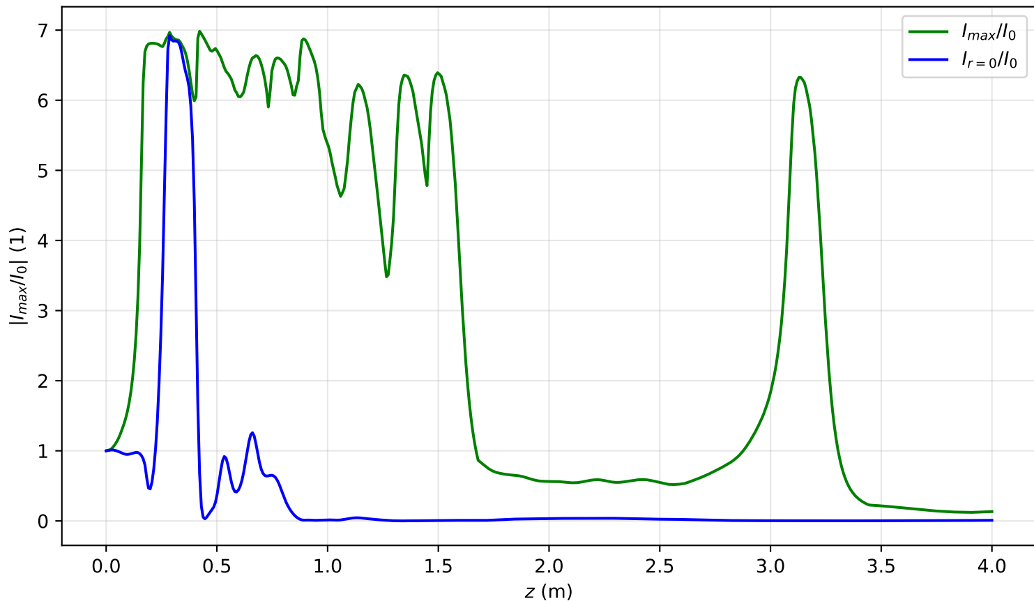
I_{\max}(x = 0, y = 0, z)/I_0 , P_{\text{in}}=16.1\text{Pcr} , noisy input, artificial time
