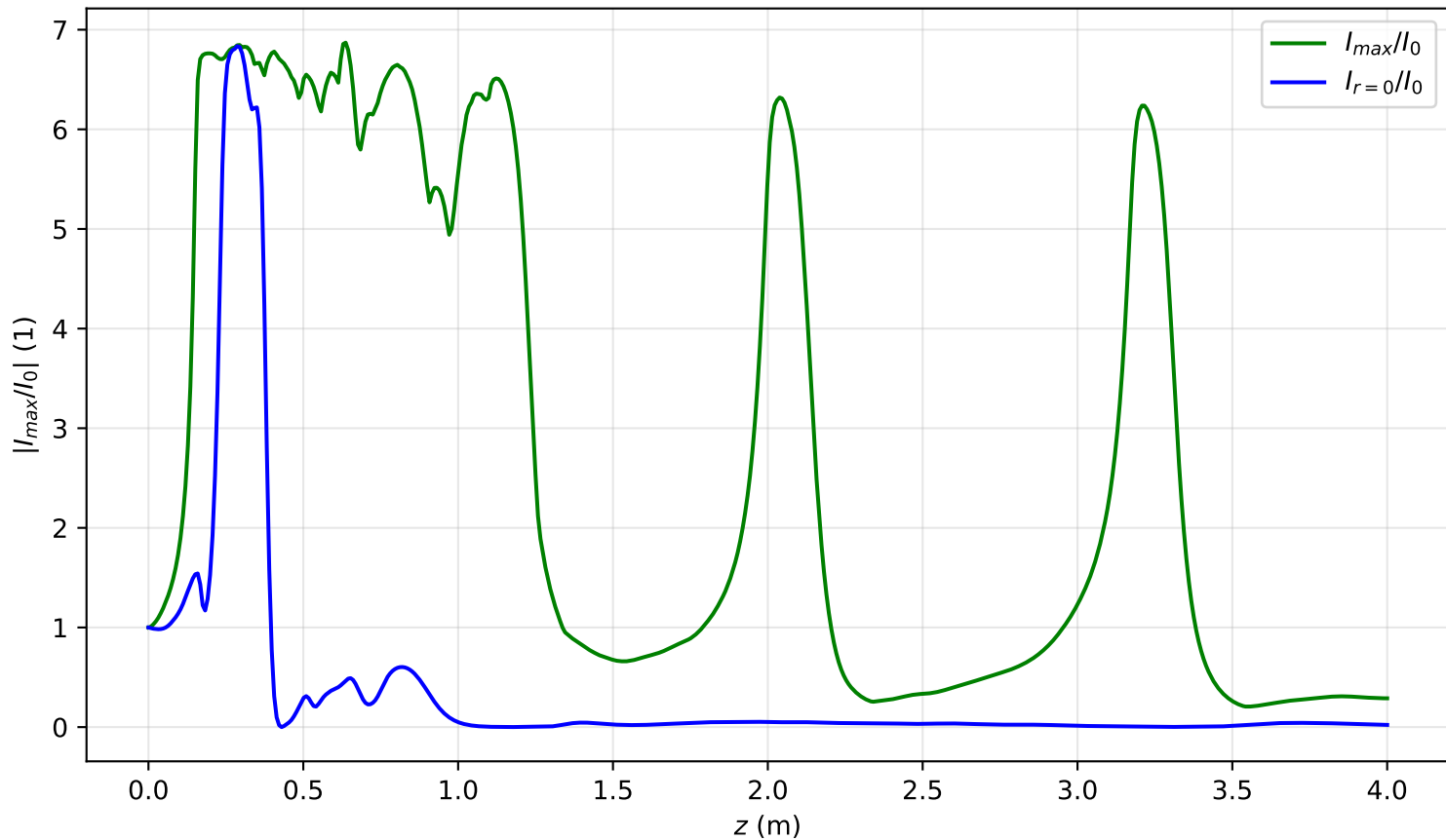
I_{max}(x = 0, y = 0, z)/I_0 , P_{in}=16.2\text{Pcr} , noisy input, artificial time
