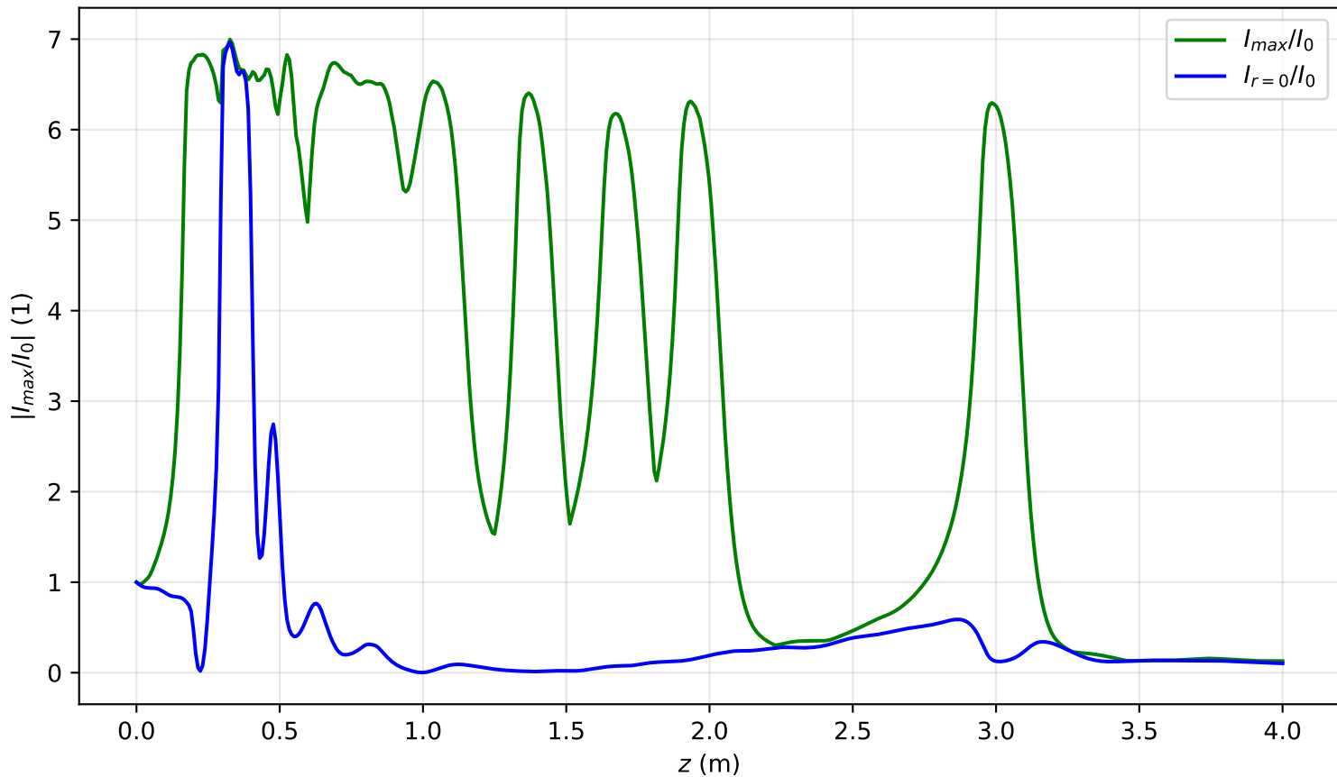
I_{max}(x = 0, y = 0, z)/I_0 , Pin=16.3Pcr, noisy input, artificial time
