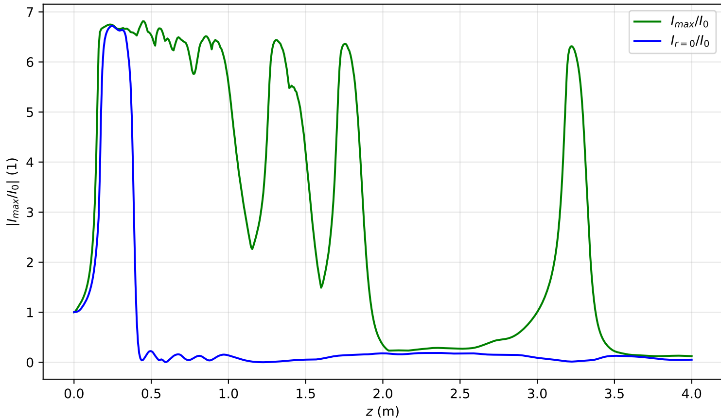
I_{max}(x = 0, y = 0, z)/I_0 , Pin=16.4Pcr, noisy input, artificial time
