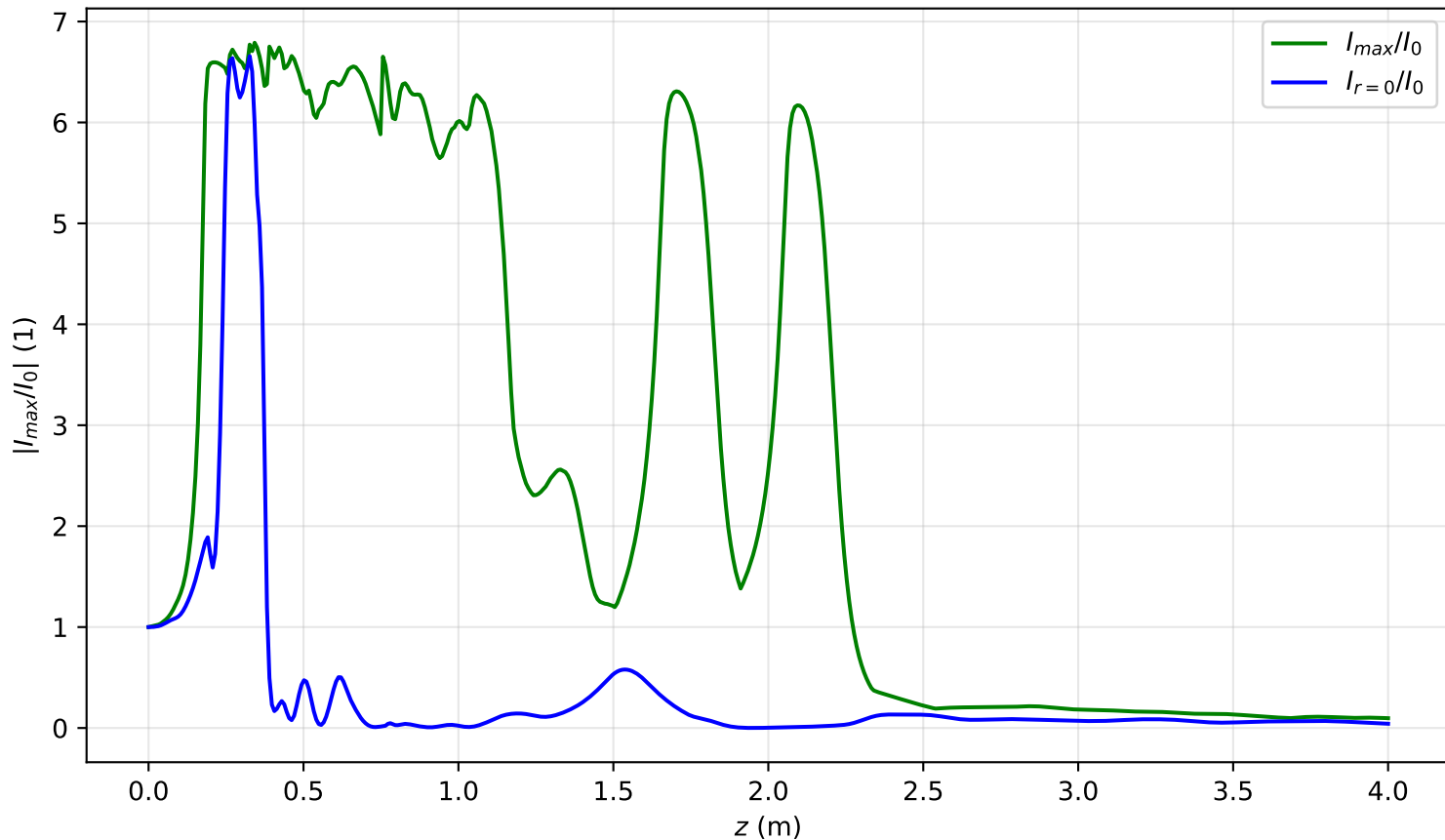
I_{max}(x = 0, y = 0, z)/I_0 , Pin=16.6Pcr, noisy input, artificial time
