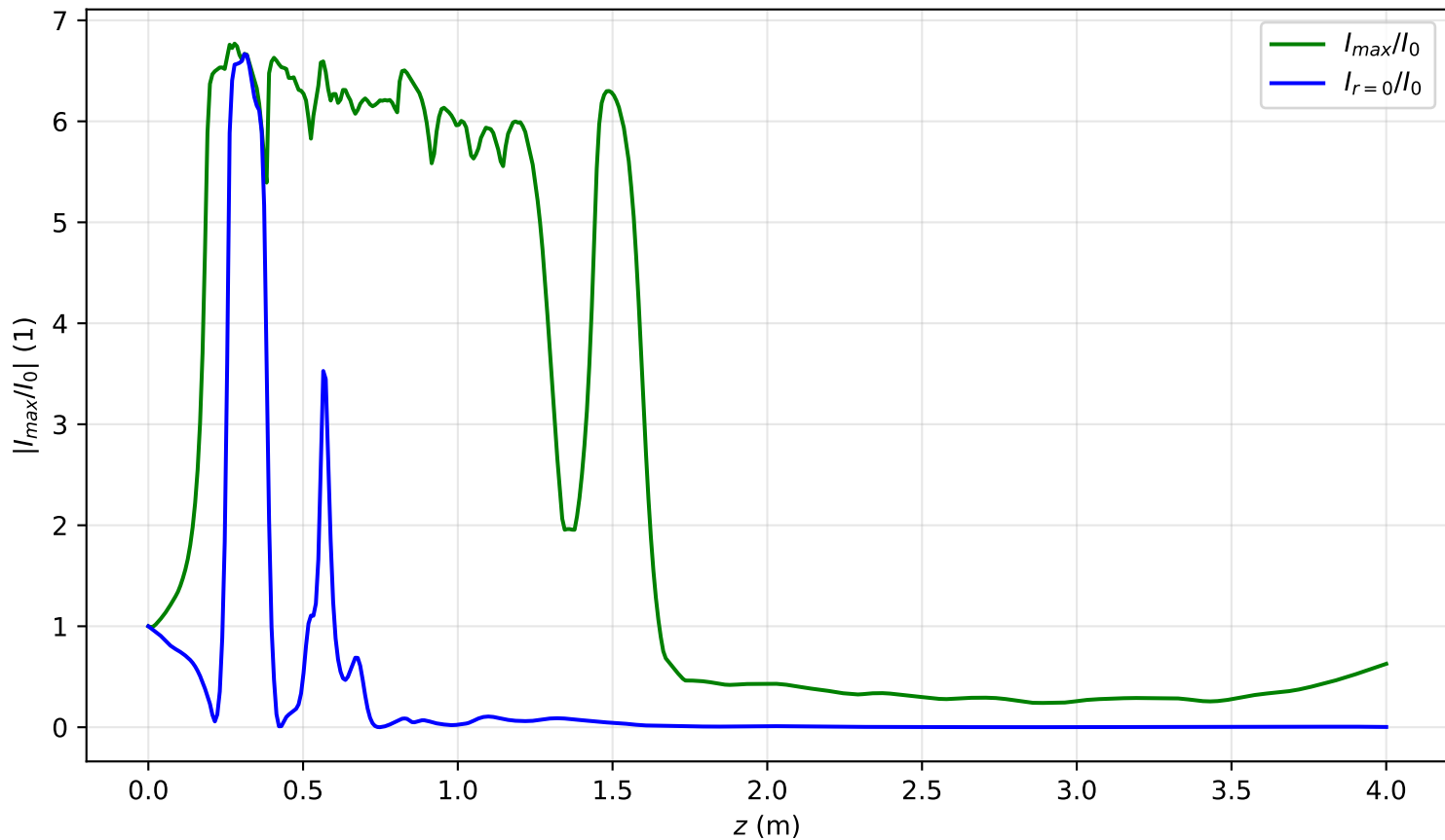
I_{max}(x = 0, y = 0, z)/I_0 , Pin=16.7Pcr, noisy input, artificial time
