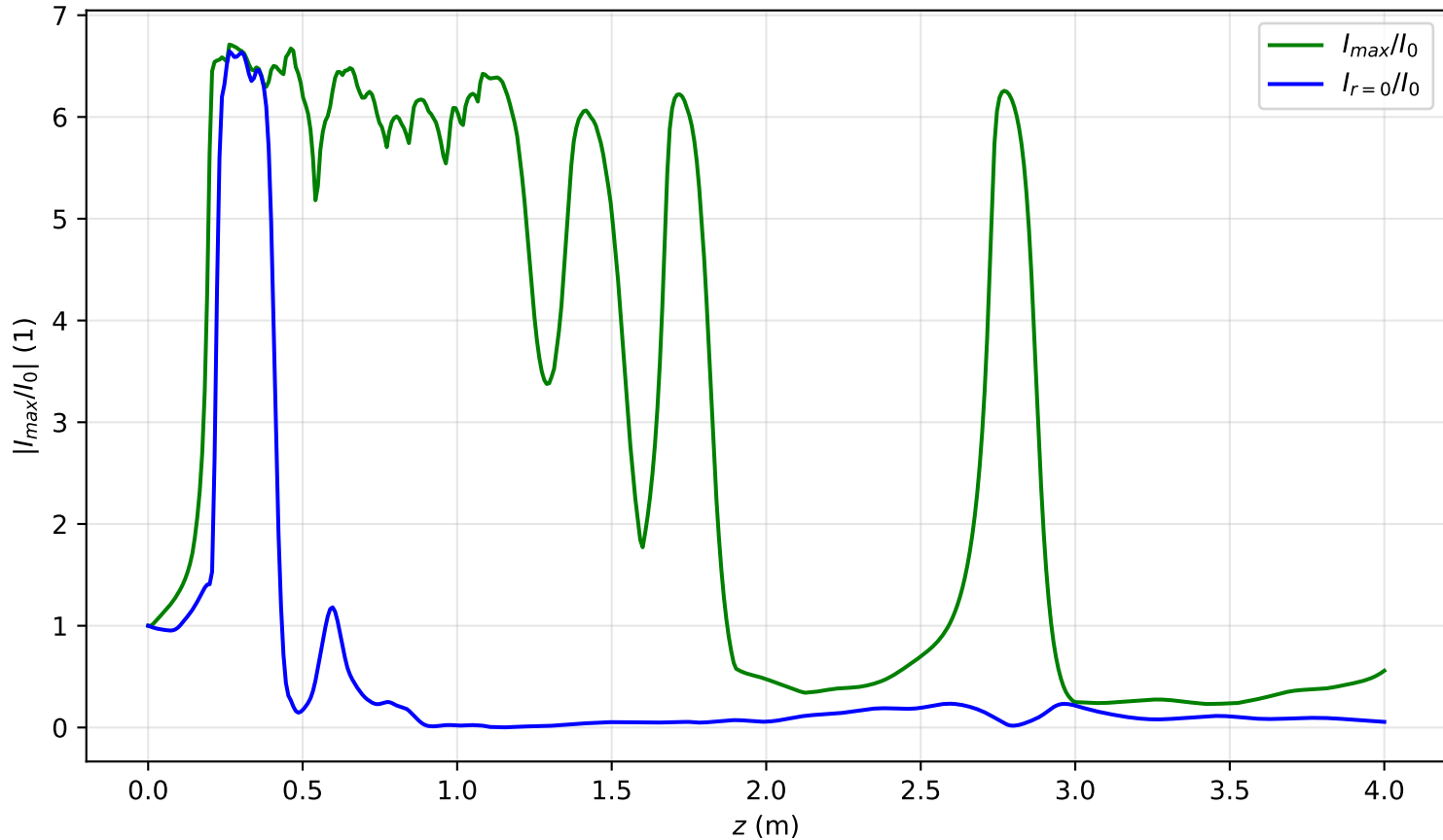
I_{max}(x = 0, y = 0, z)/I_0 , Pin=16.8Pcr, noisy input, artificial time
