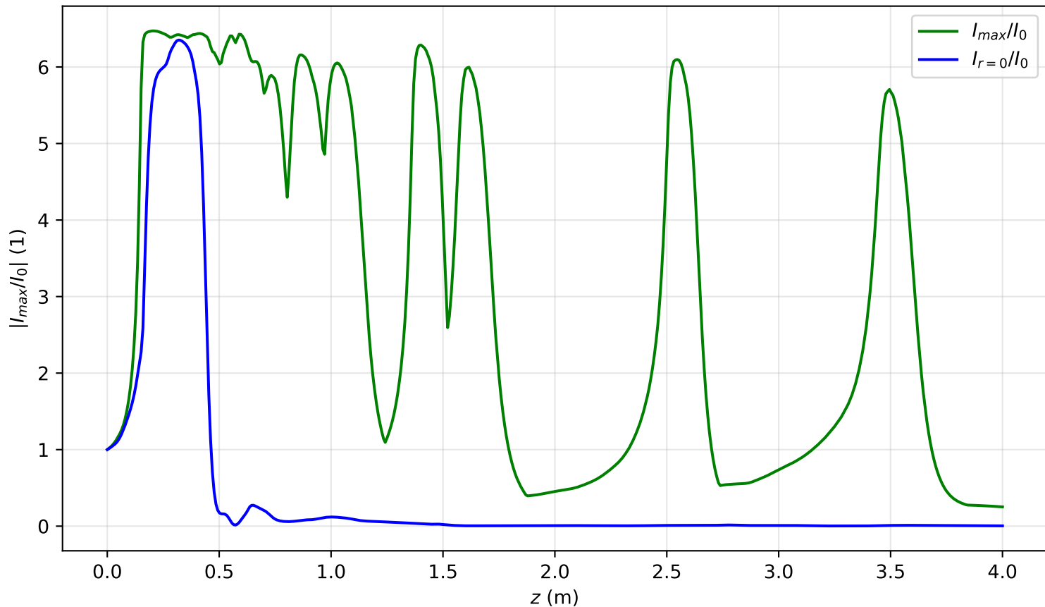
I_{max}(x = 0, y = 0, z)/I_0 , Pin=17.0Pcr, noisy input, artificial time
