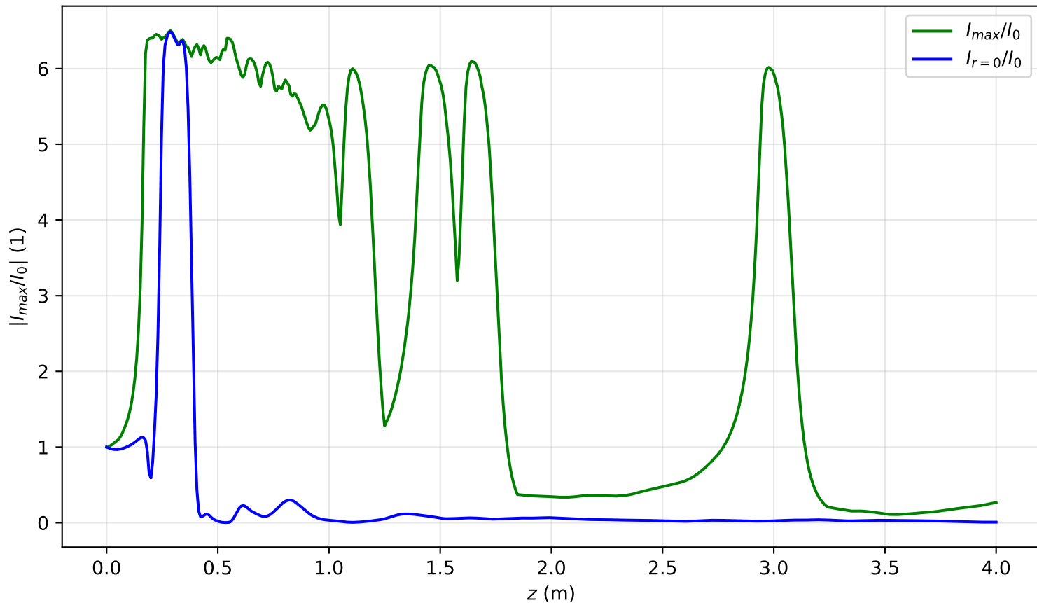
I_{max}(x = 0, y = 0, z)/I_0 , Pin=17.2Pcr, noisy input, artificial time
