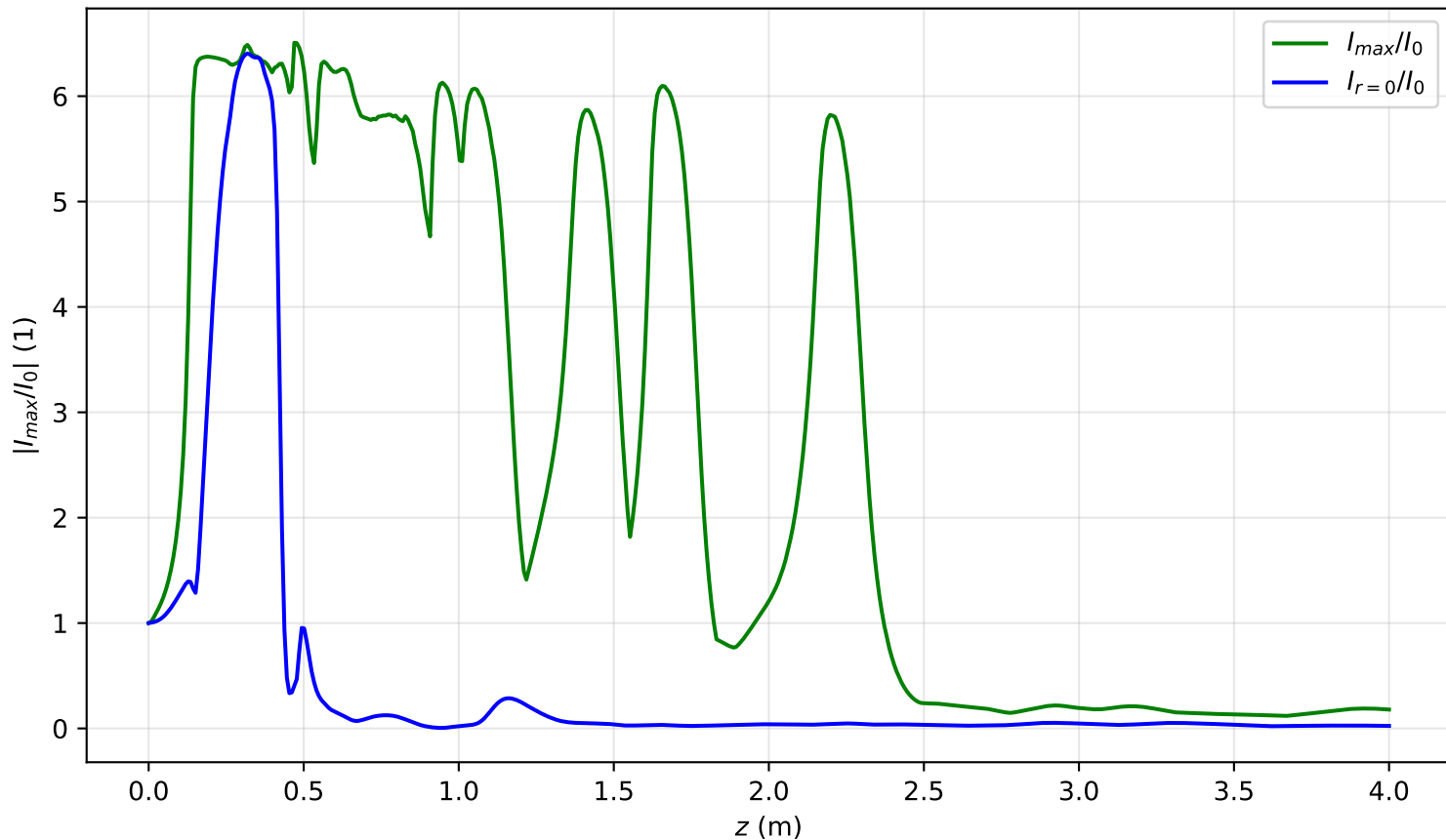
I_{max}(x = 0, y = 0, z)/I_0 , Pin=17.3Pcr, noisy input, artificial time
