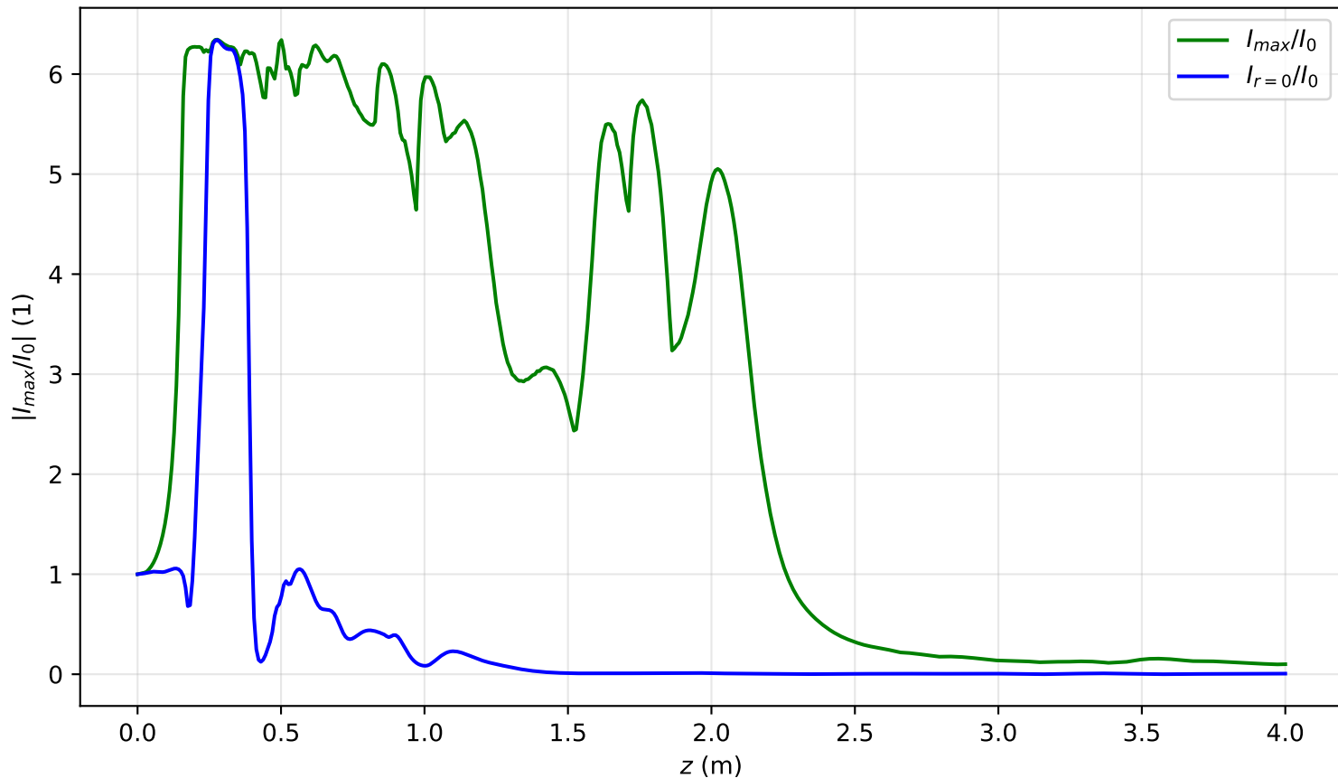
I_{max}(x = 0, y = 0, z)/I_0 , Pin=17.5Pcr, noisy input, artificial time
