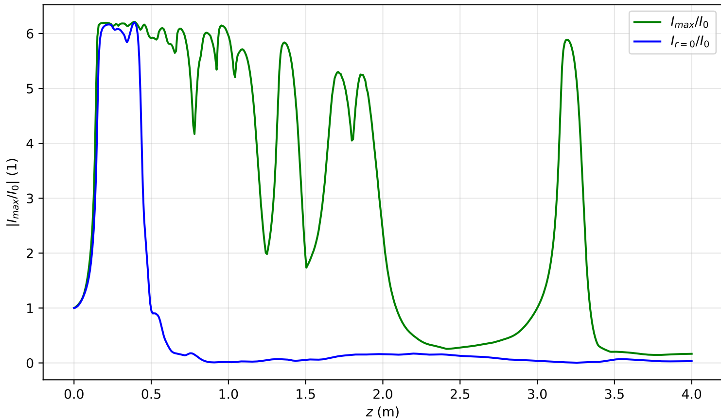
I_{max}(x = 0, y = 0, z)/I_0 , P_{in}=17.8P_{cr} , noisy input, artificial time
