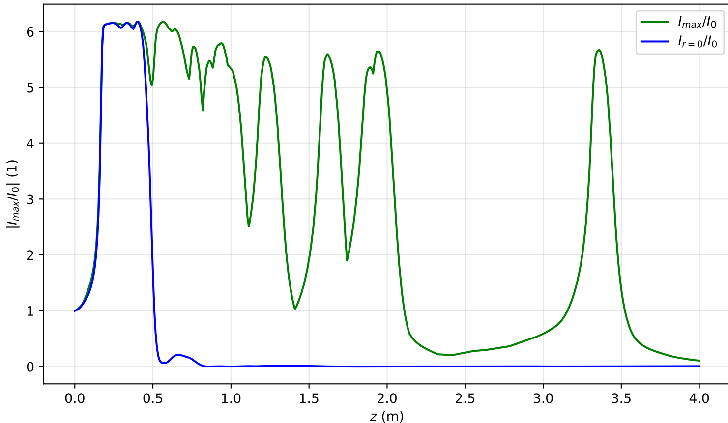
I_{\max}(x = 0, y = 0, z)/I_0 , P_{\text{in}}=17.9\text{Pcr} , noisy input, artificial time
