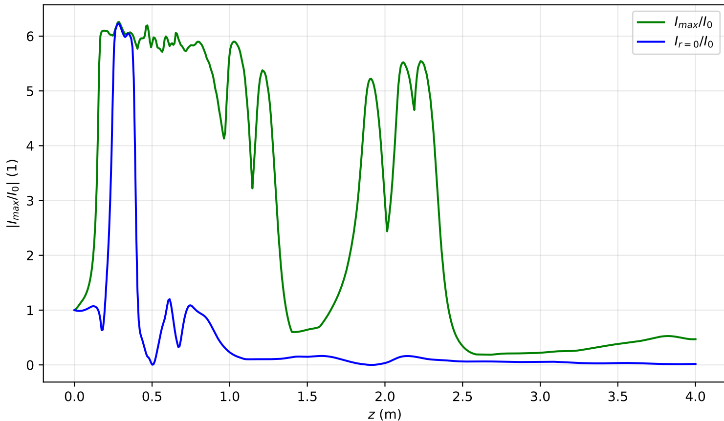
I_{max}(x = 0, y = 0, z)/I_0 , P_{in}=18.0\text{Pcr} , noisy input, artificial time
