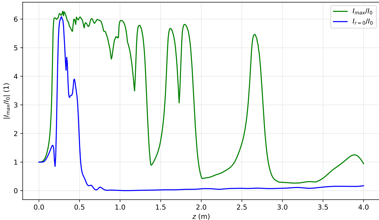
I_{max}(x = 0, y = 0, z)/I_0 , P_{in}=18.1\text{Pcr} , noisy input, artificial time
