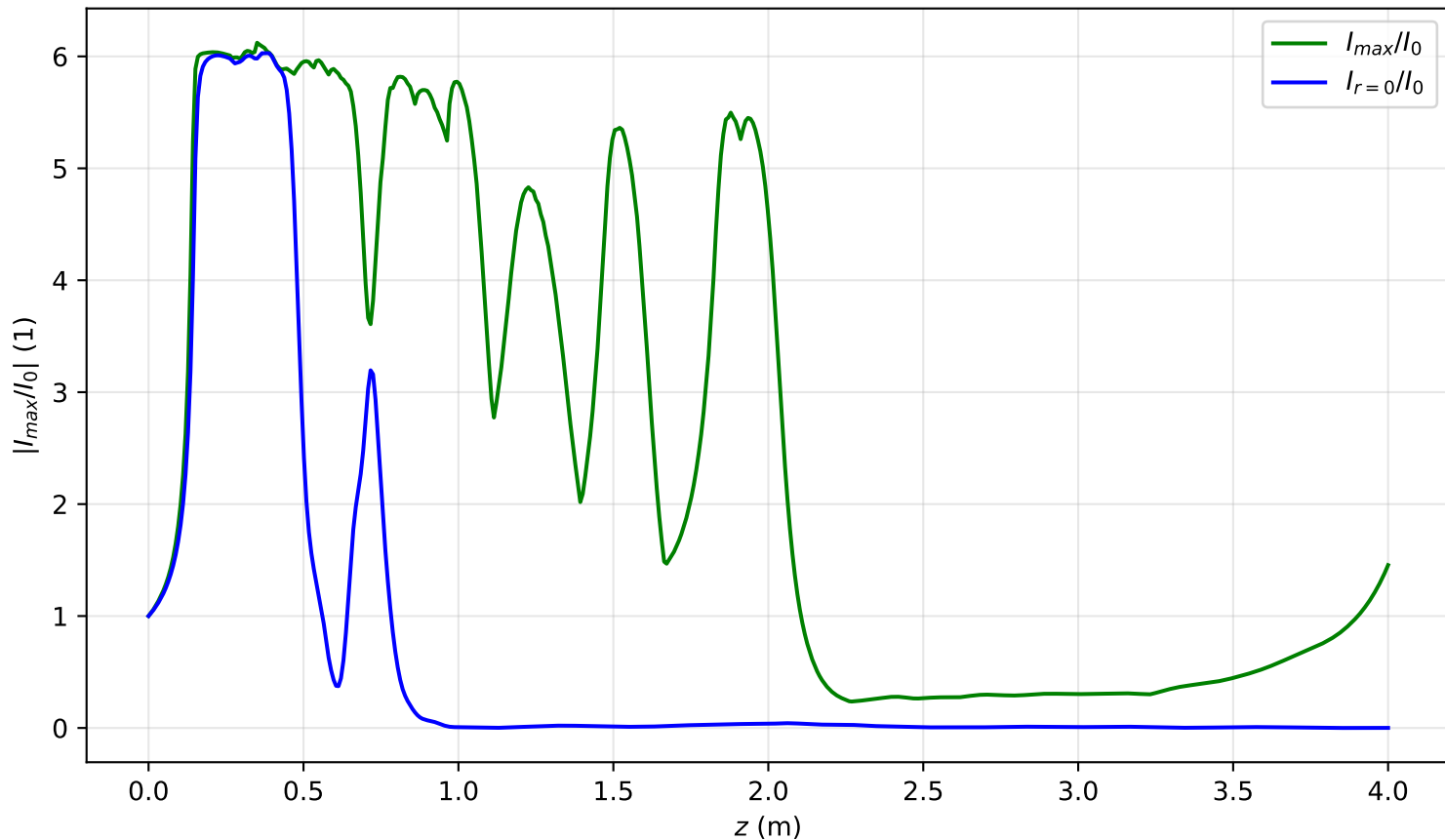
I_{\max}(x = 0, y = 0, z)/I_0 , Pin=18.2Pcr, noisy input, artificial time
