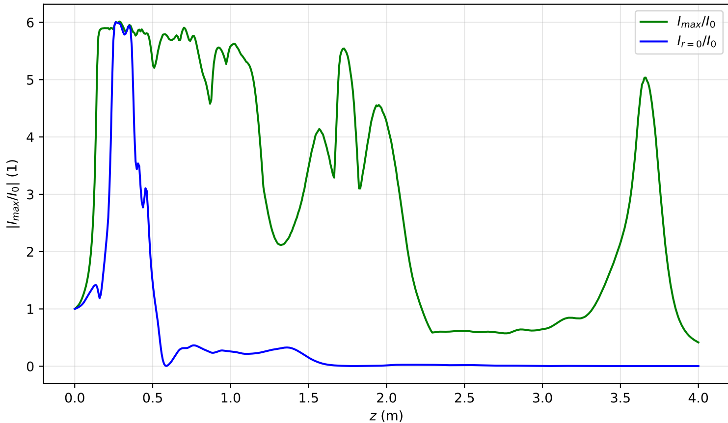
I_{max}(x = 0, y = 0, z)/I_0 , Pin=18.5Pcr, noisy input, artificial time
