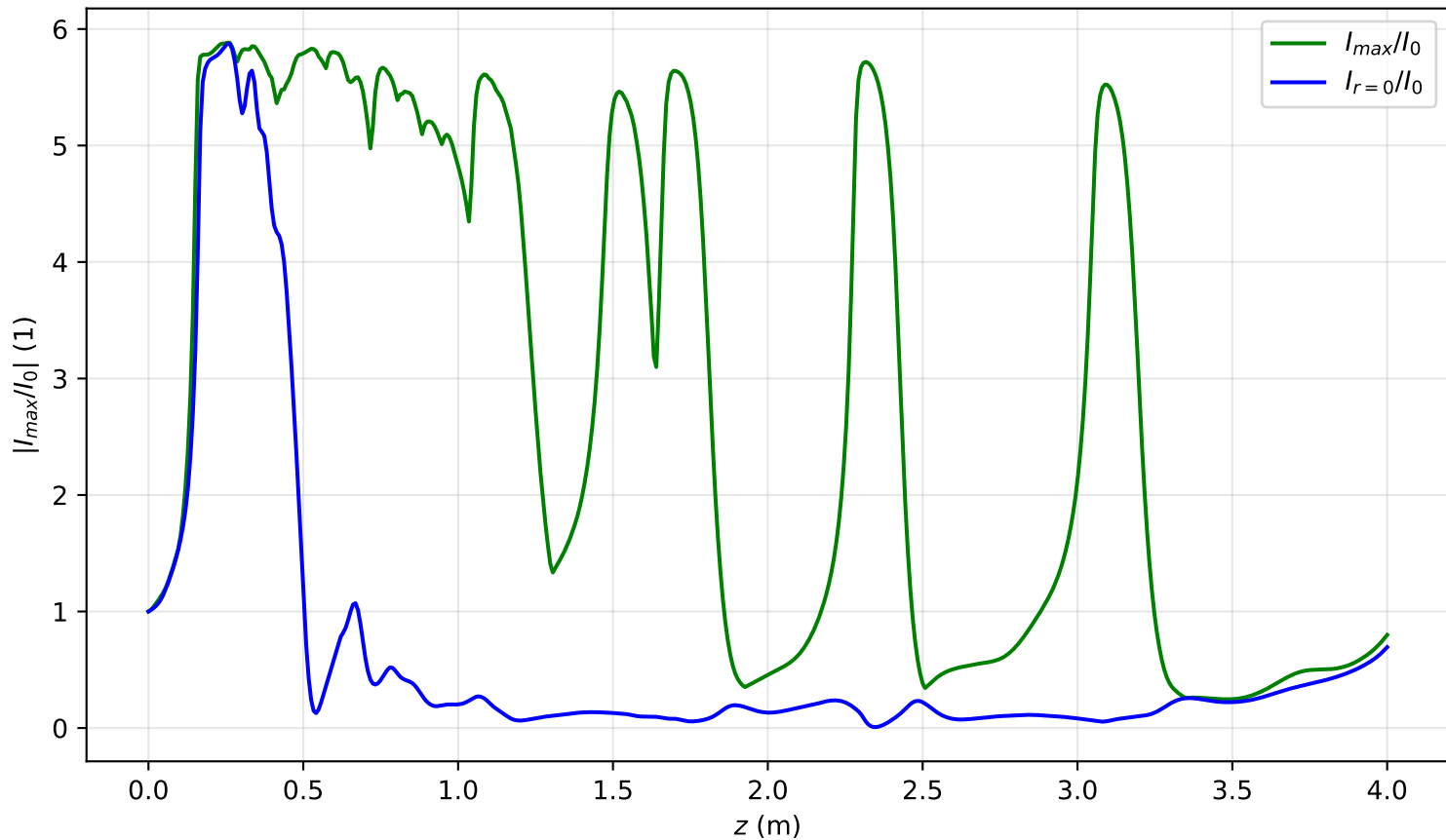
I_{max}(x = 0, y = 0, z)/I_0 , Pin=18.8Pcr, noisy input, artificial time
