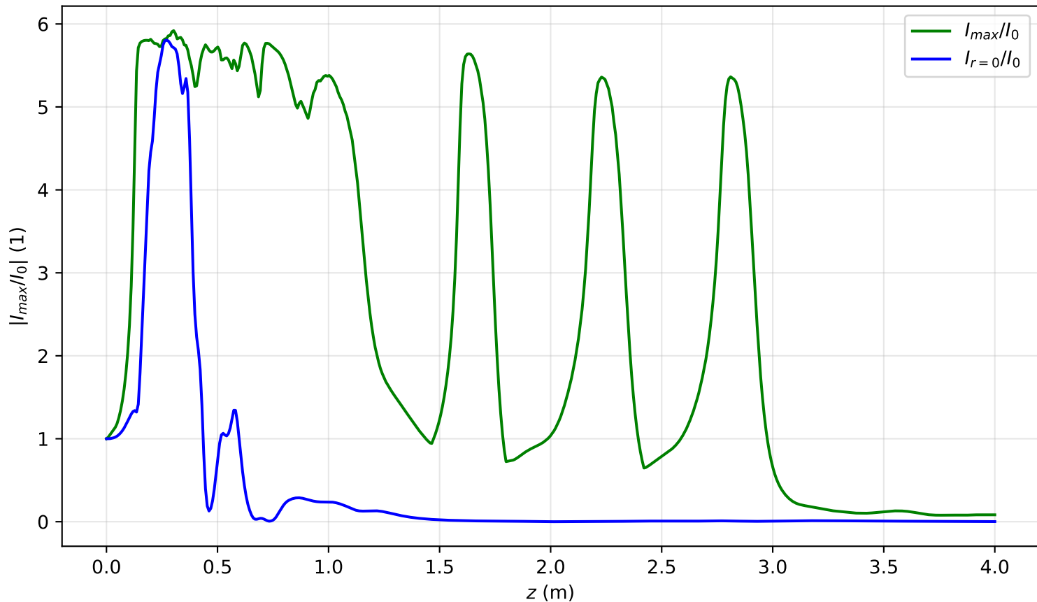
I_{max}(x = 0, y = 0, z)/I_0 , Pin=18.9Pcr, noisy input, artificial time
