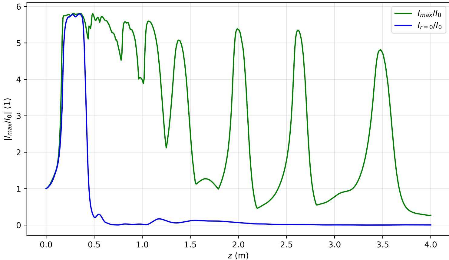
I_{\max}(x = 0, y = 0, z)/I_0 , Pin=19.0Pcr, noisy input, artificial time
