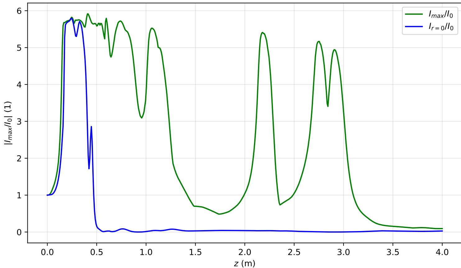
I_{max}(x = 0, y = 0, z)/I_0 , Pin=19.1Pcr, noisy input, artificial time
