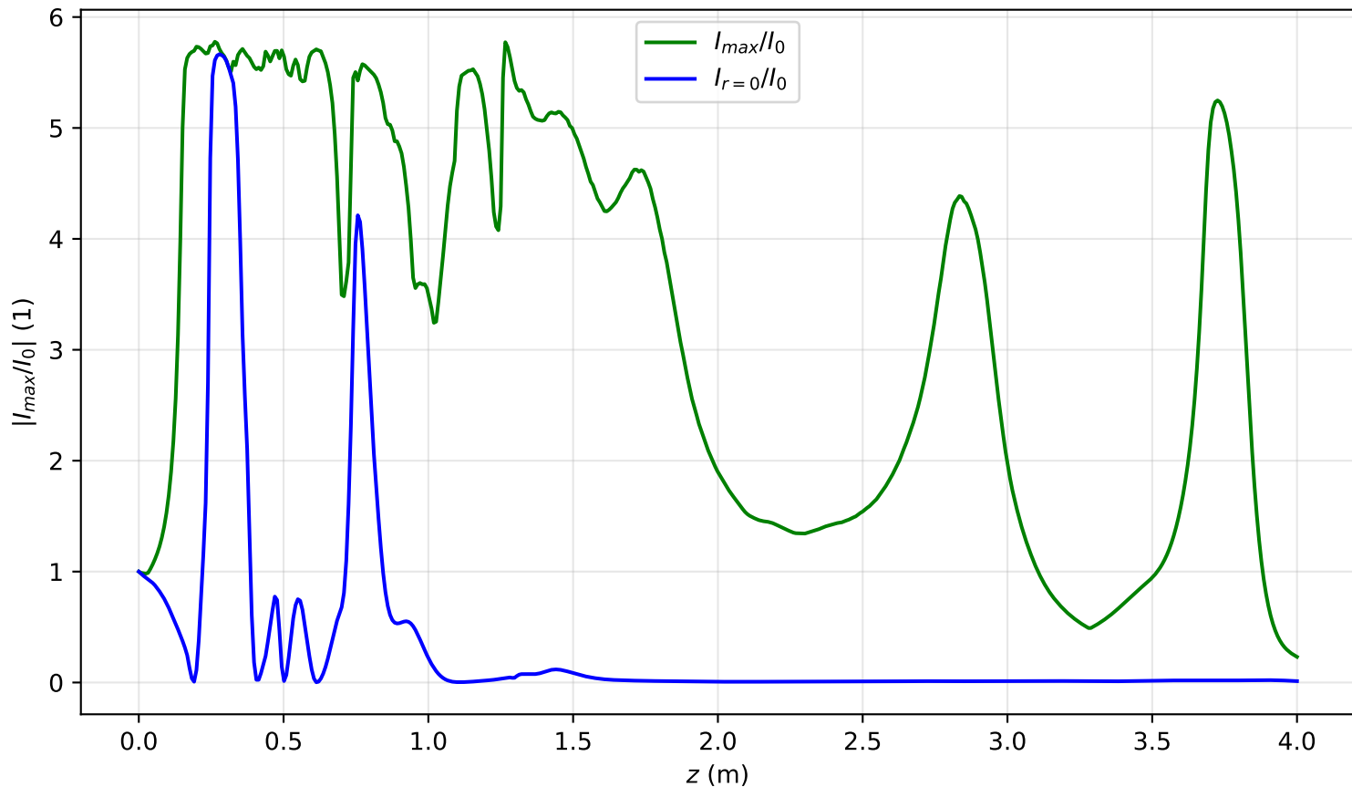
I_{max}(x=0, y=0, z)/I_0 , Pin=19.2Pcr, noisy input, artificial time
