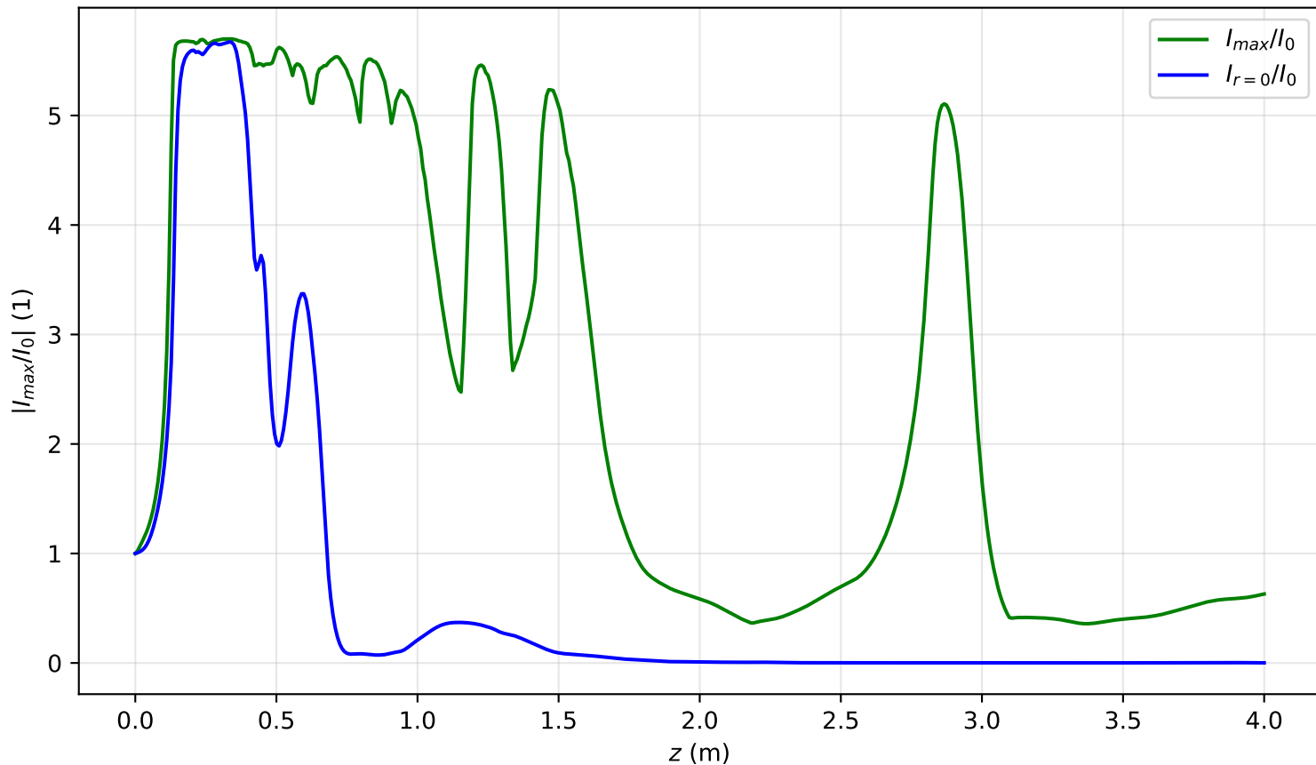
I_{\max}(x = 0, y = 0, z)/I_0 , Pin=19.3Pcr, noisy input, artificial time
