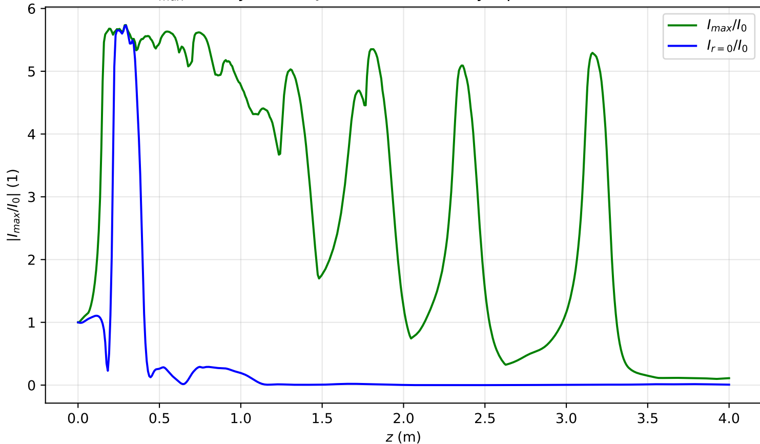
I_{max}(x = 0, y = 0, z)/I_0 , Pin=19.4Pcr, noisy input, artificial time
