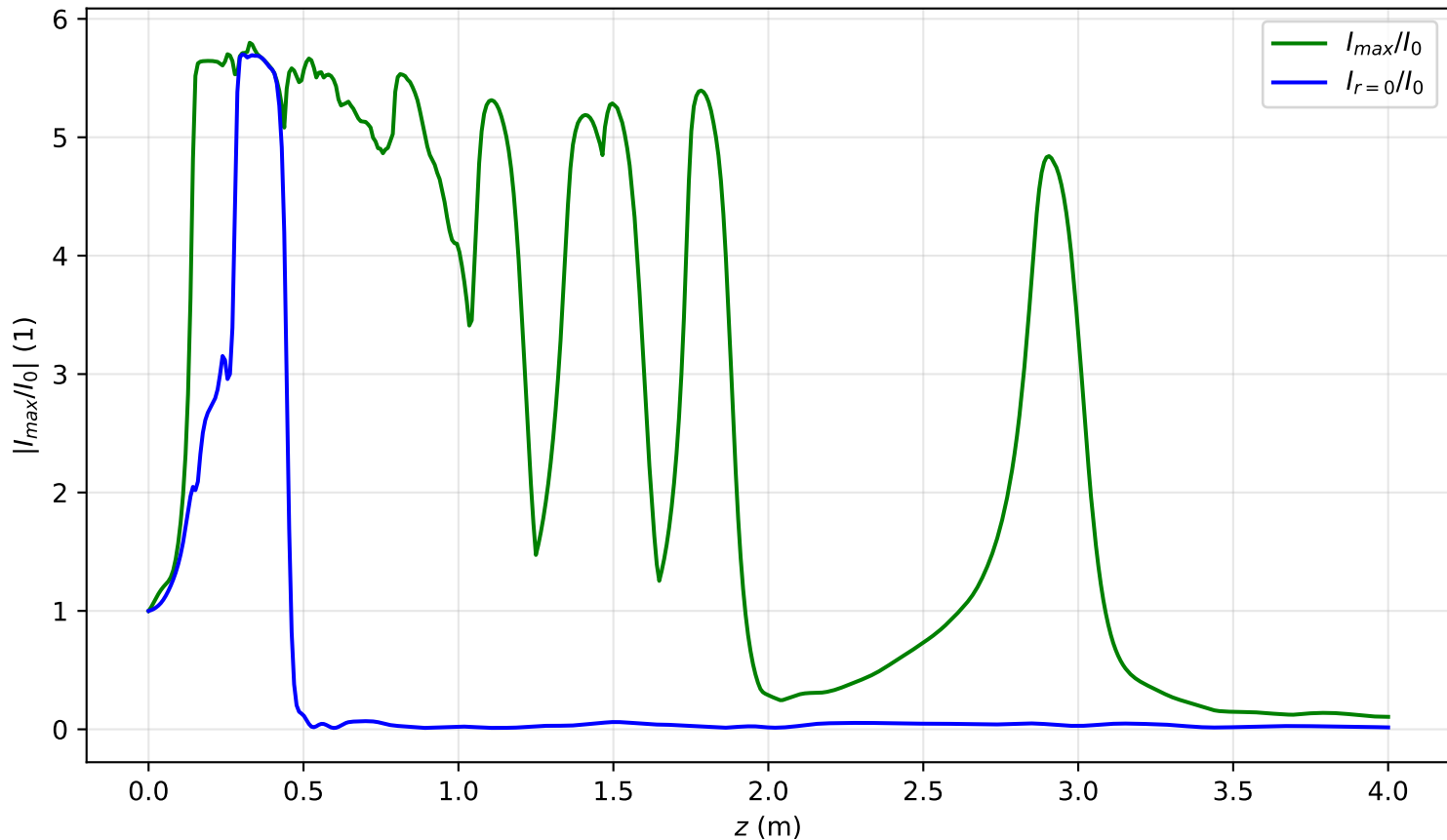
I_{max}(x = 0, y = 0, z)/I_0 , Pin=19.5Pcr, noisy input, artificial time
