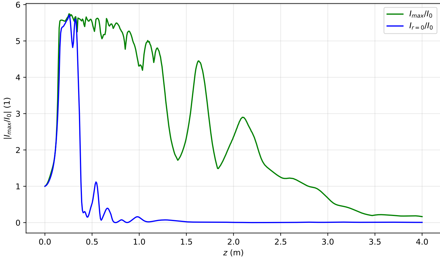
I_{max}(x = 0, y = 0, z)/I_0 , P_{in}=19.7\text{Pcr} , noisy input, artificial time
